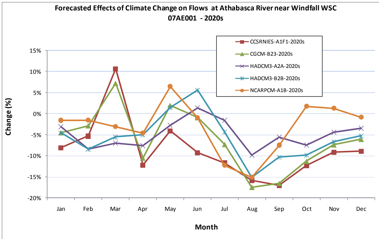
Figure 5.3 Forecasted Effects of Climate Change on Simulated Mean Monthly Flows – 2020s Scenarios (continued)
