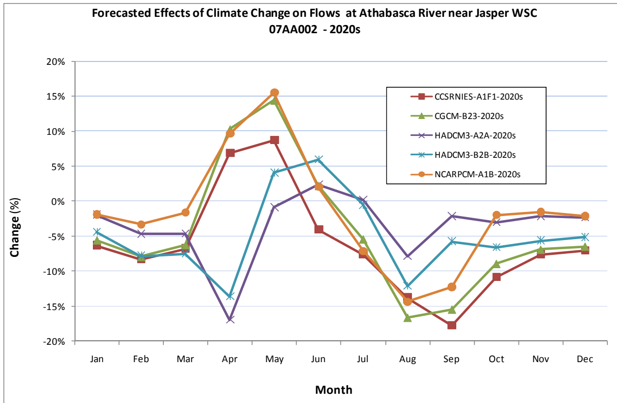
Figure 5.3 Forecasted Effects of Climate Change on Simulated Mean Monthly Flows – 2020s Scenarios
