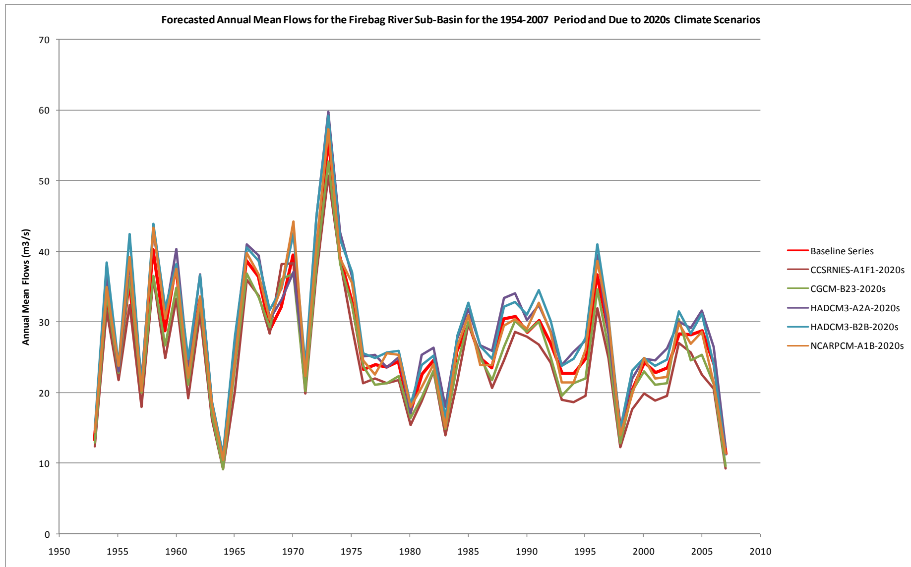
Figure 5.6 Baseline and Future Annual Flow Series for the Firebag River Sub-Basin
