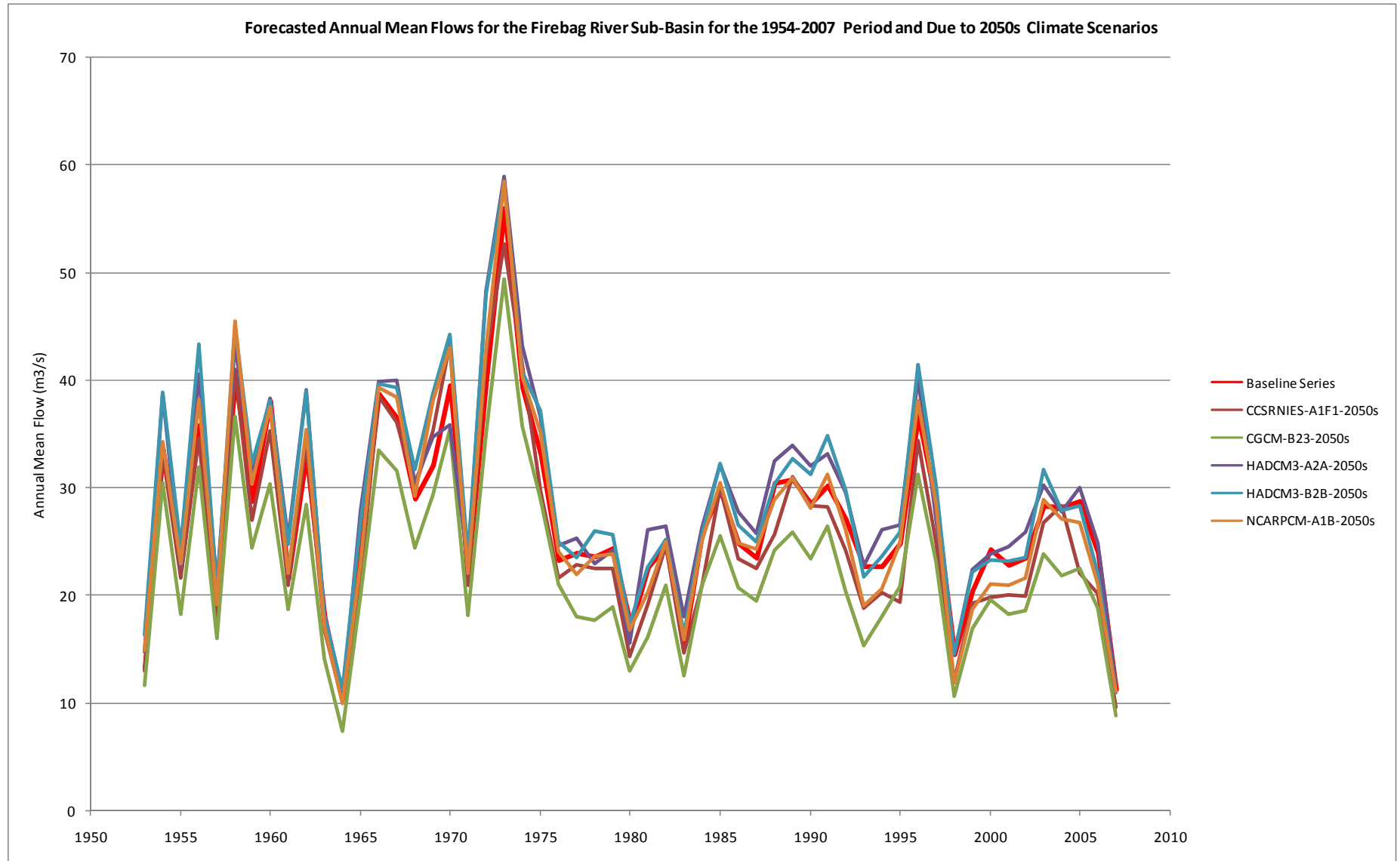
Figure 5.6 Baseline and Future Annual Flow Series for the Firebag River Sub-Basin (continued)
