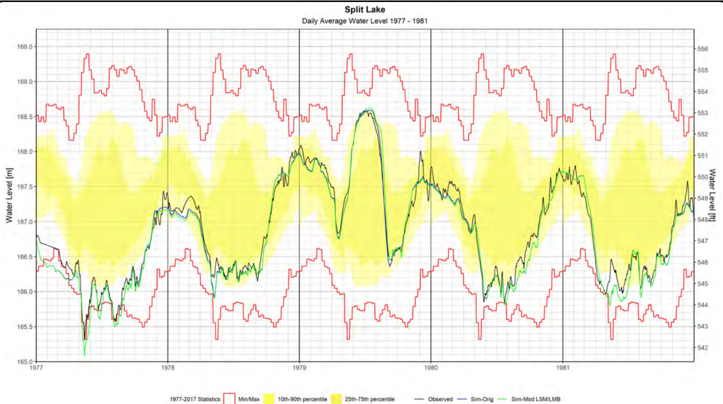
Figure 14: Split Lake 1977-1981
