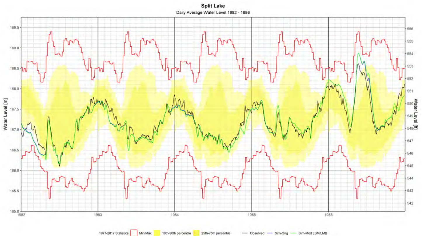
Figure 15: Split Lake 1982-1986
