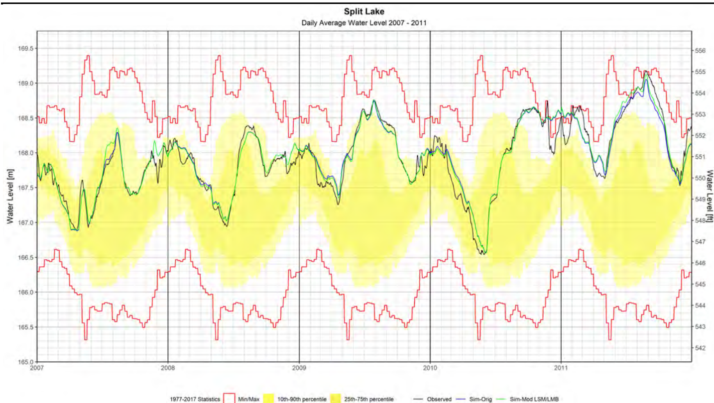
Figure 20: Split Lake 2007-2011
