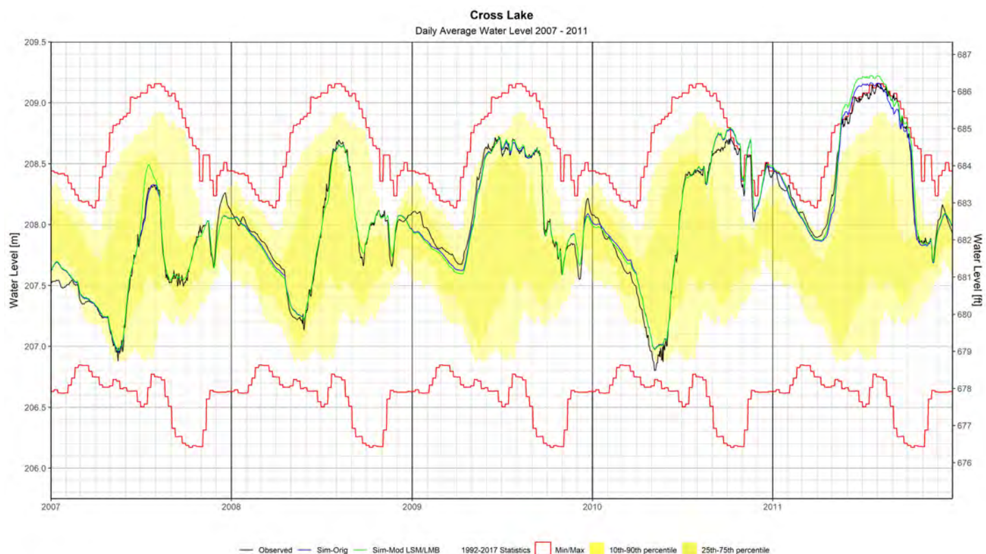
Figure 12: Cross Lake 2007-2011
