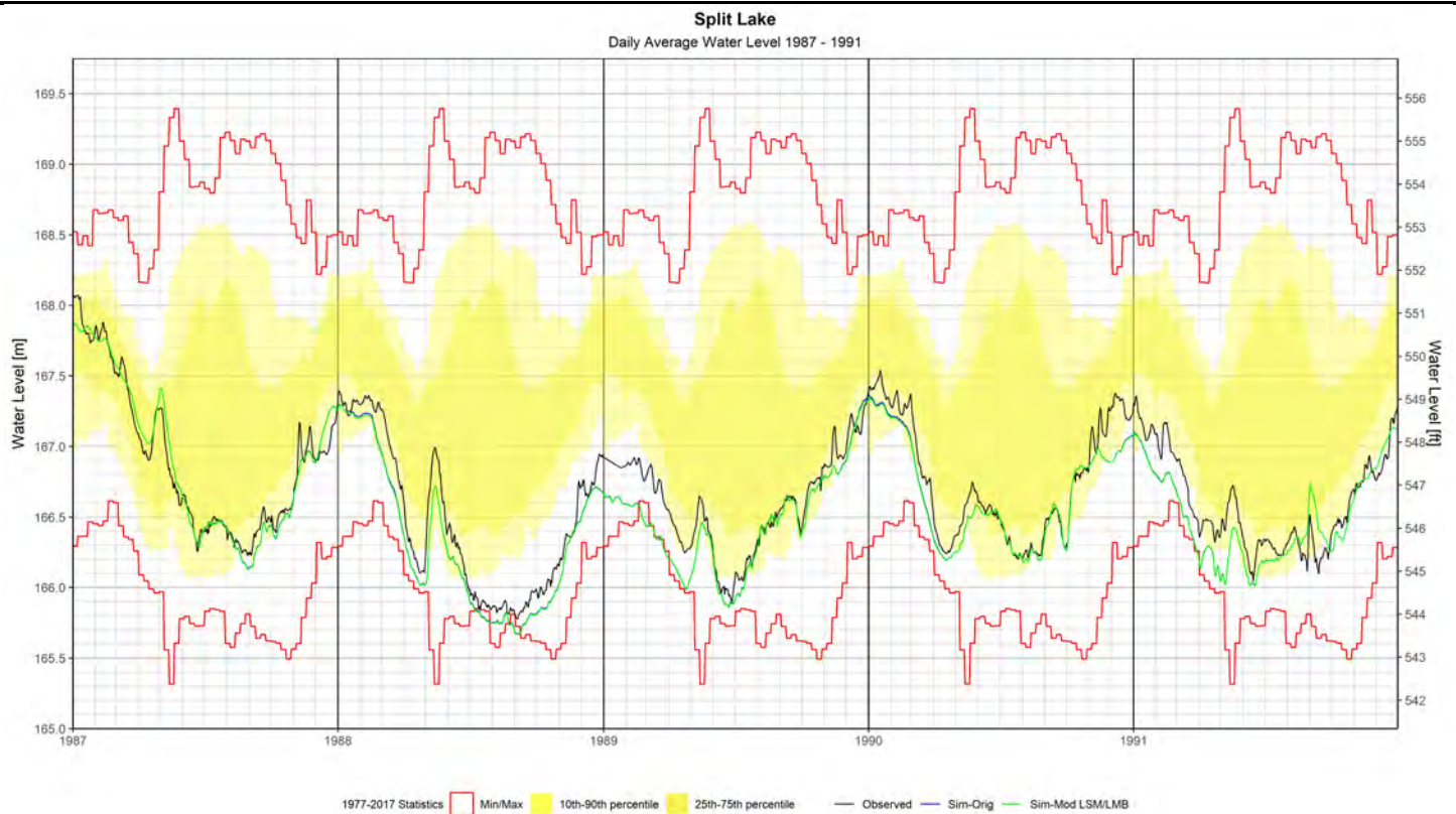
Figure 16: Split Lake 1987-1991
