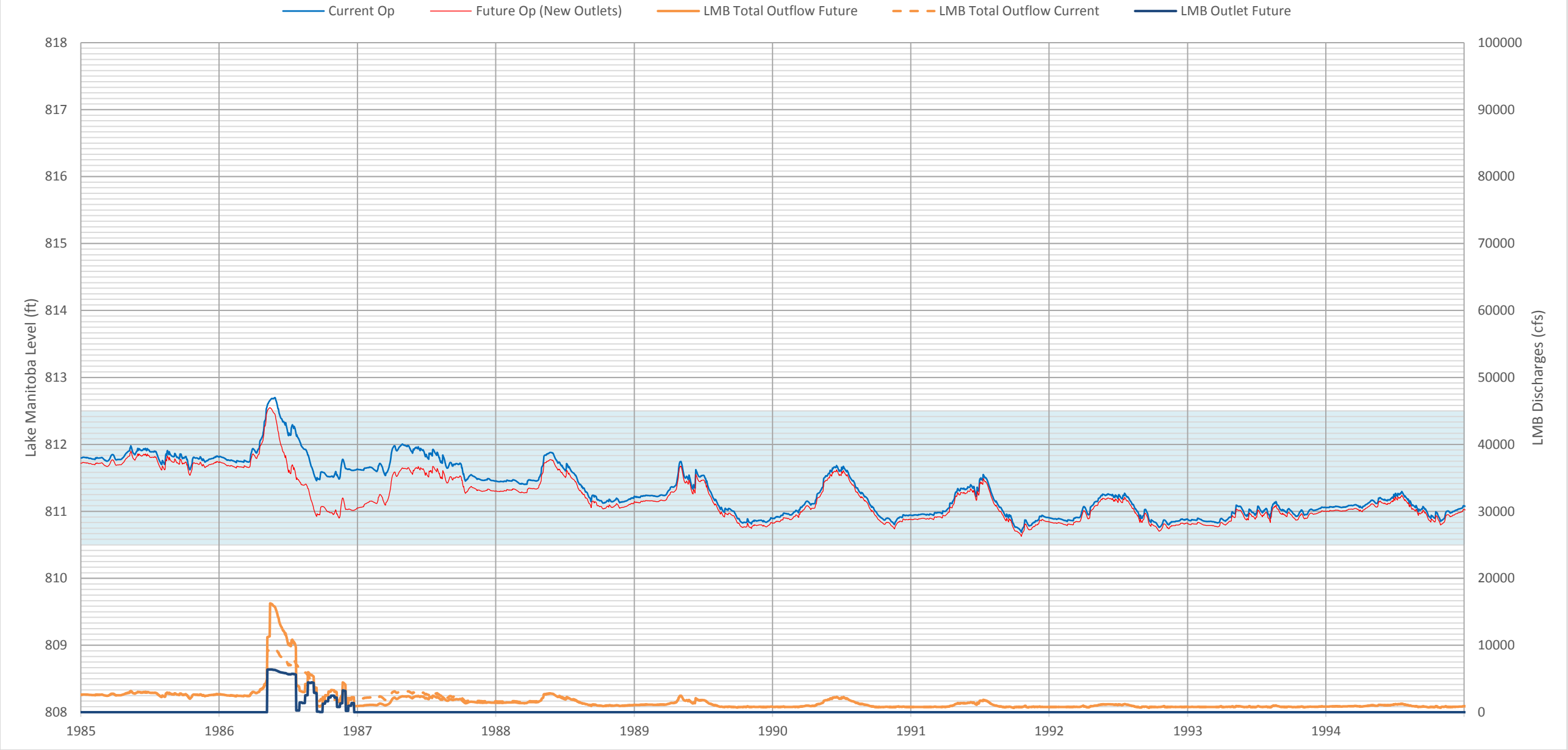
Lake Manitoba Water Level Simulations 1985 - 1994
