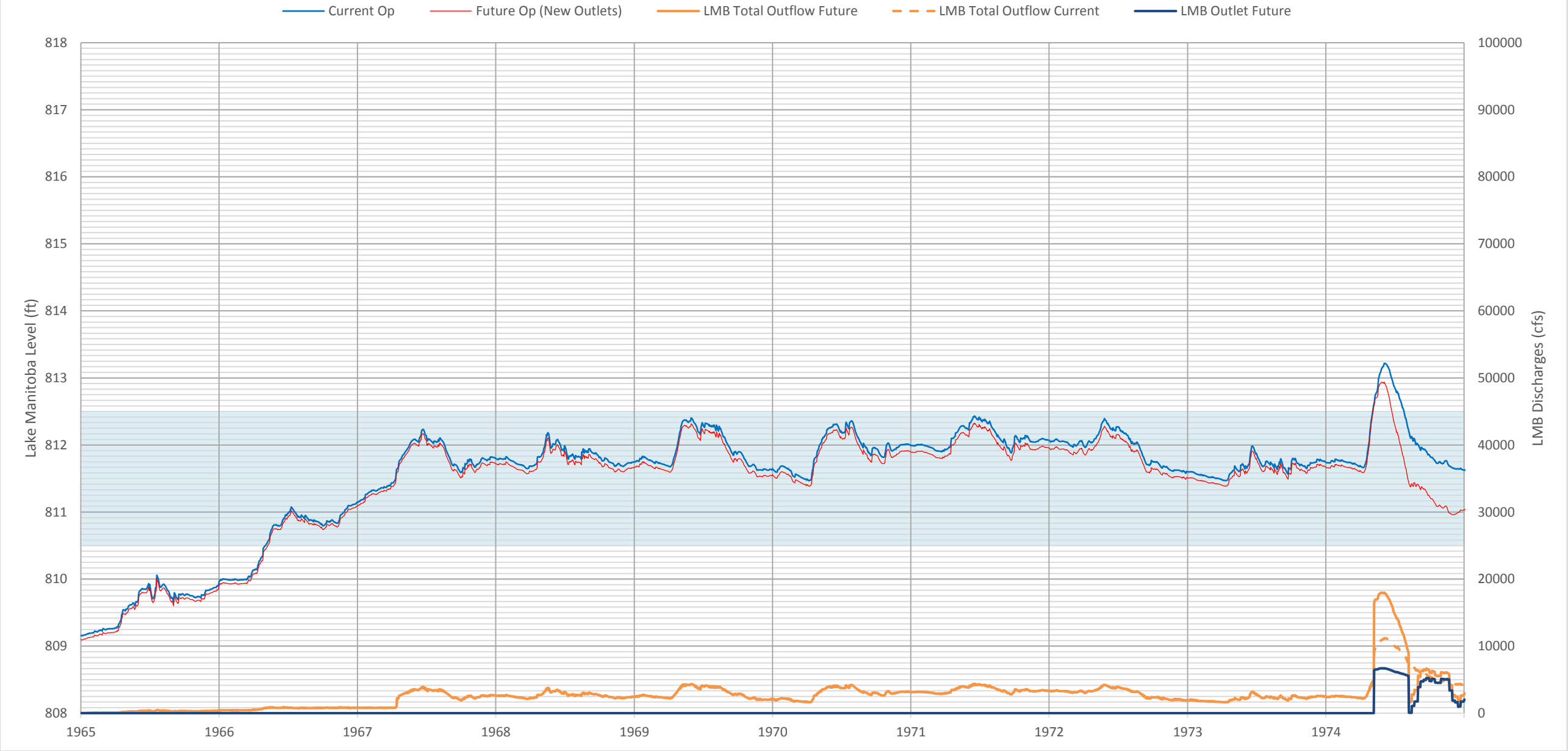
Lake Manitoba Water Level Simulations 1965 - 1974
