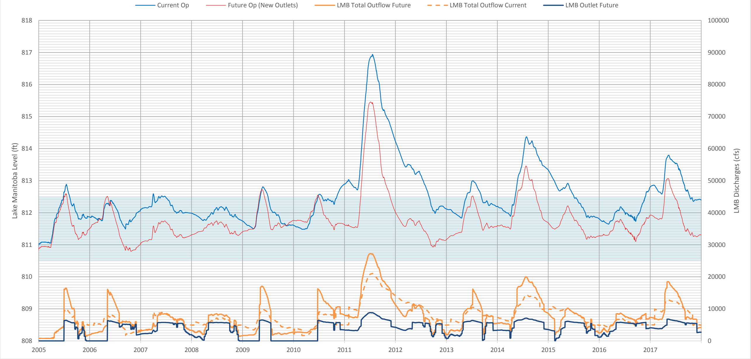
Lake Manitoba Water Level Simulations 2005 - 2017
