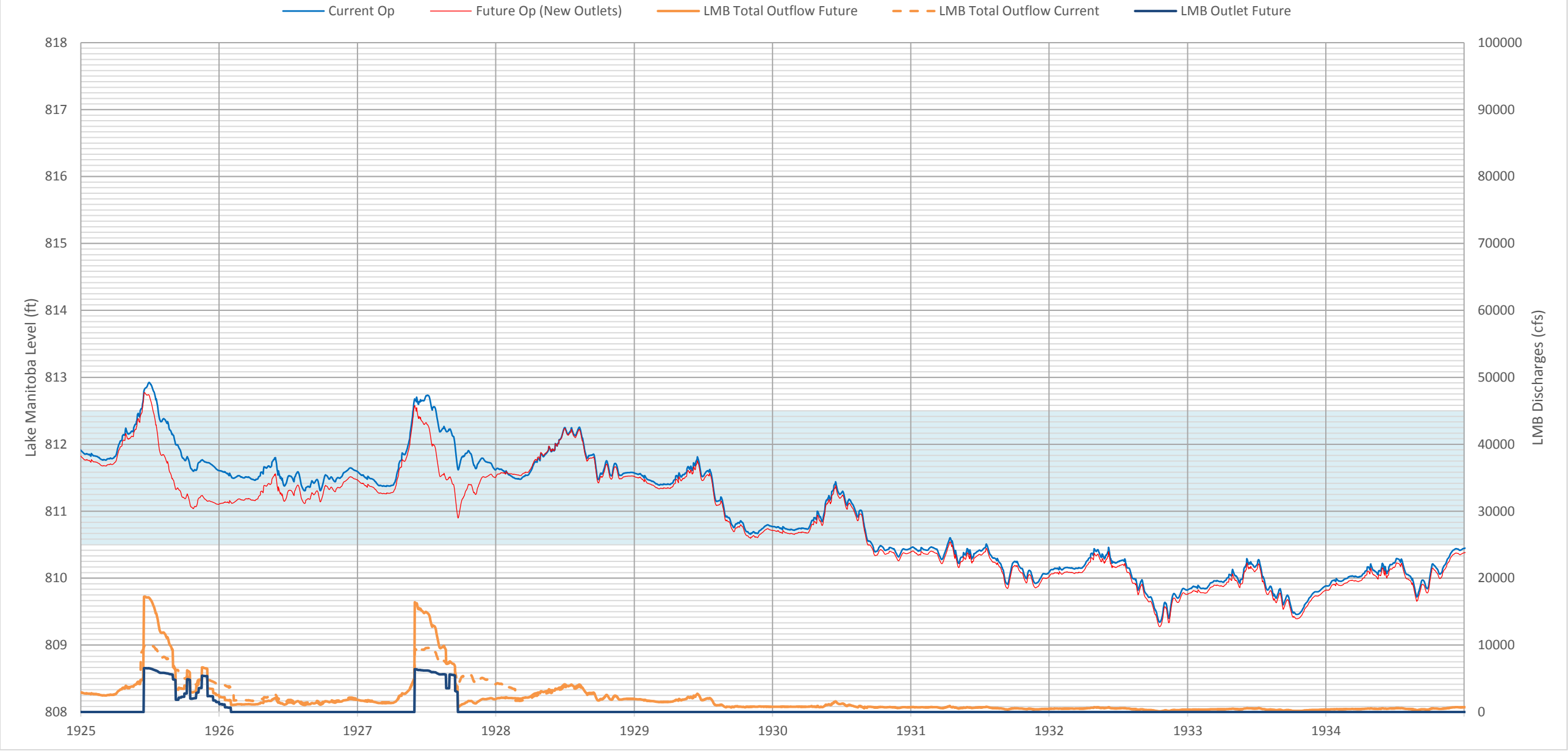
Lake Manitoba Water Level Simulations 1925 - 1934
