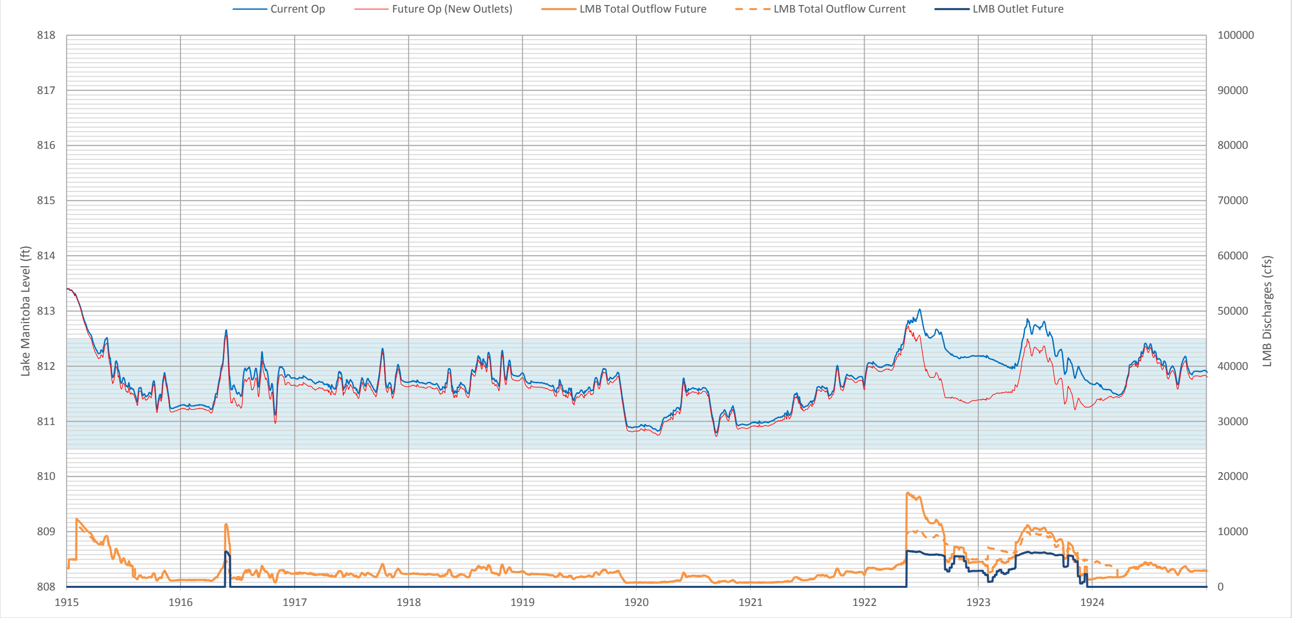
Lake Manitoba Water Level Simulations 1915-1924
