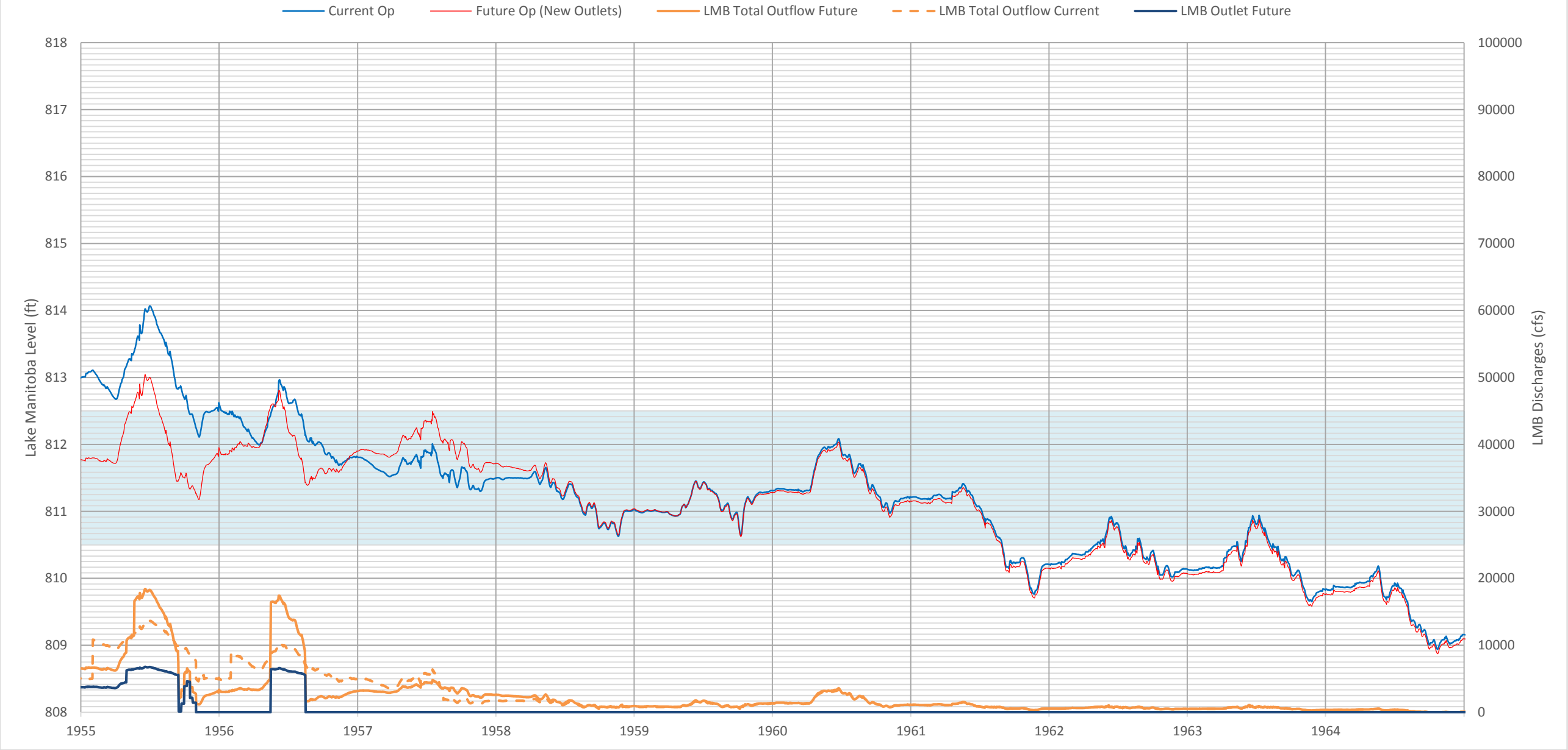
Lake Manitoba Water Level Simulations 1955 - 1964
