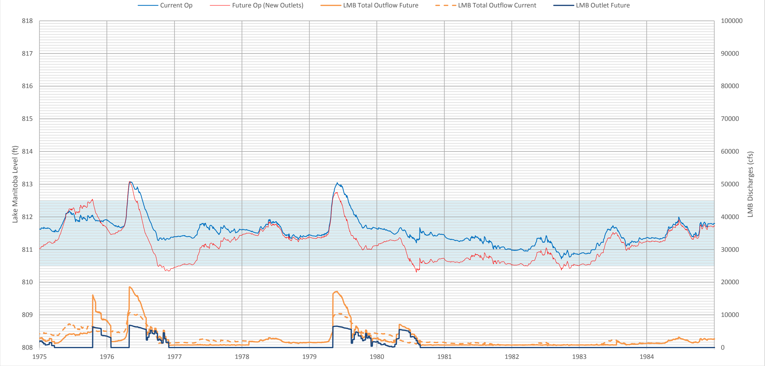
Lake Manitoba Water Level Simulations 1975 - 1984
