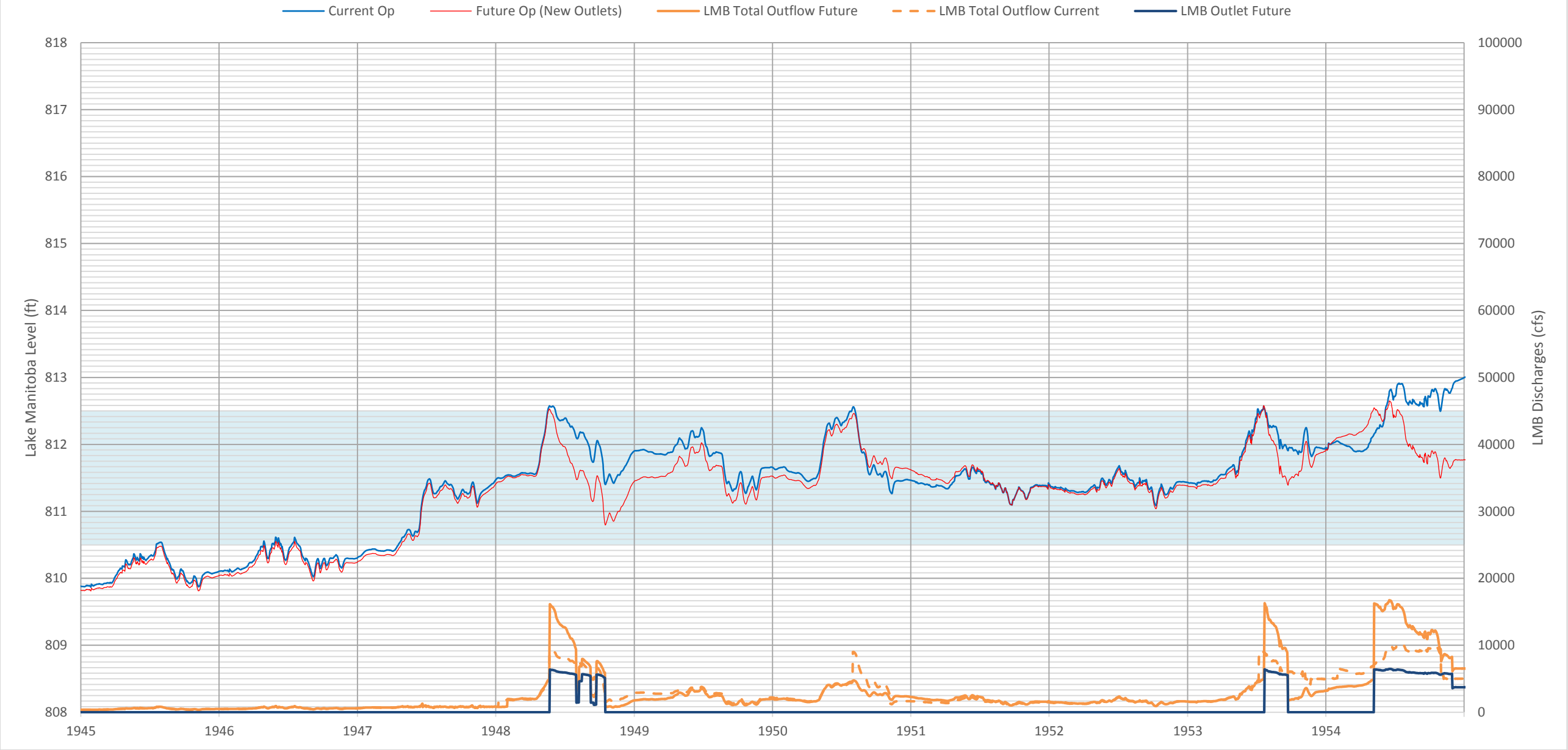
Lake Manitoba Water Level Simulations 1945 - 1954
