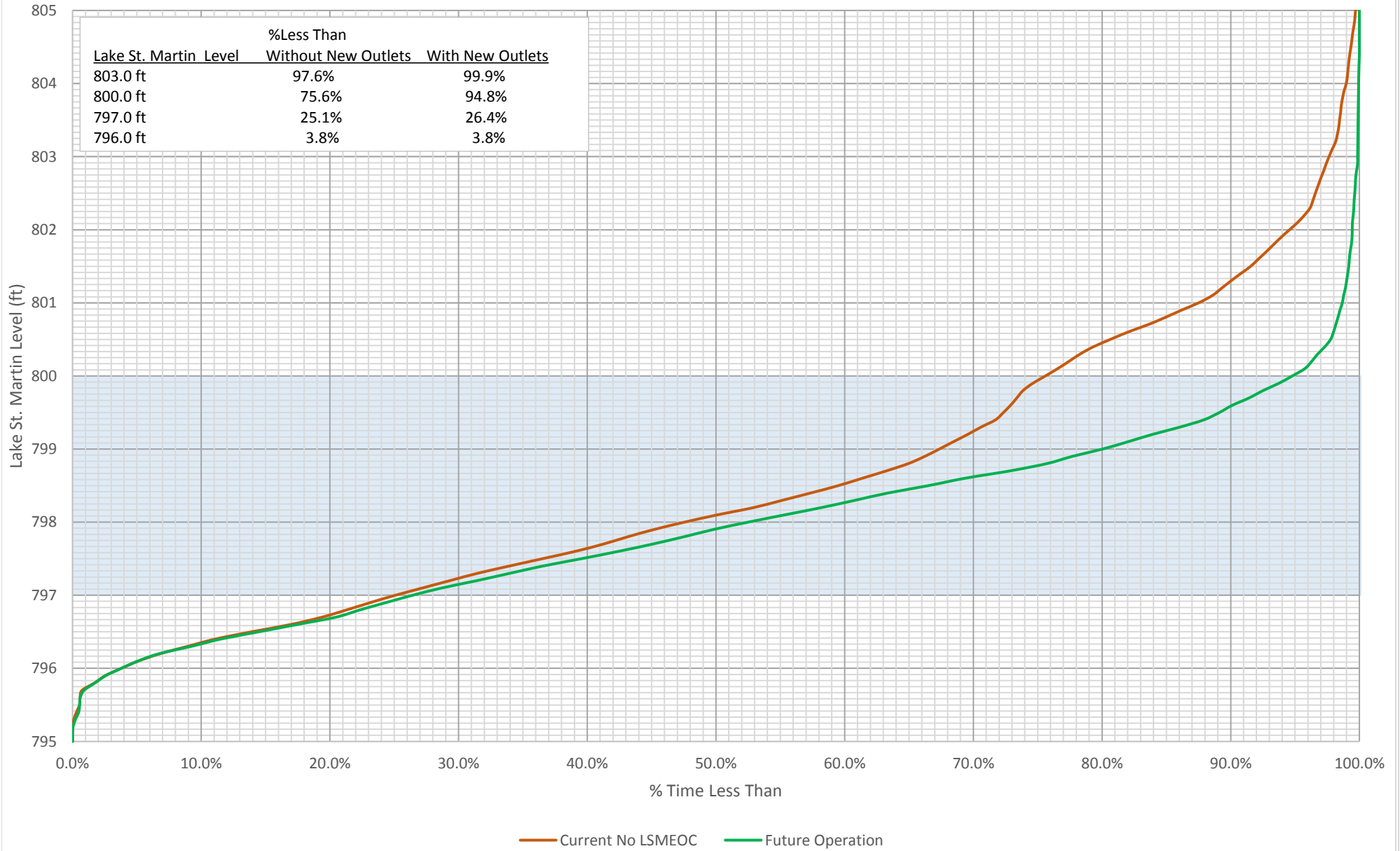
Lake St. Martin Duration Curves
