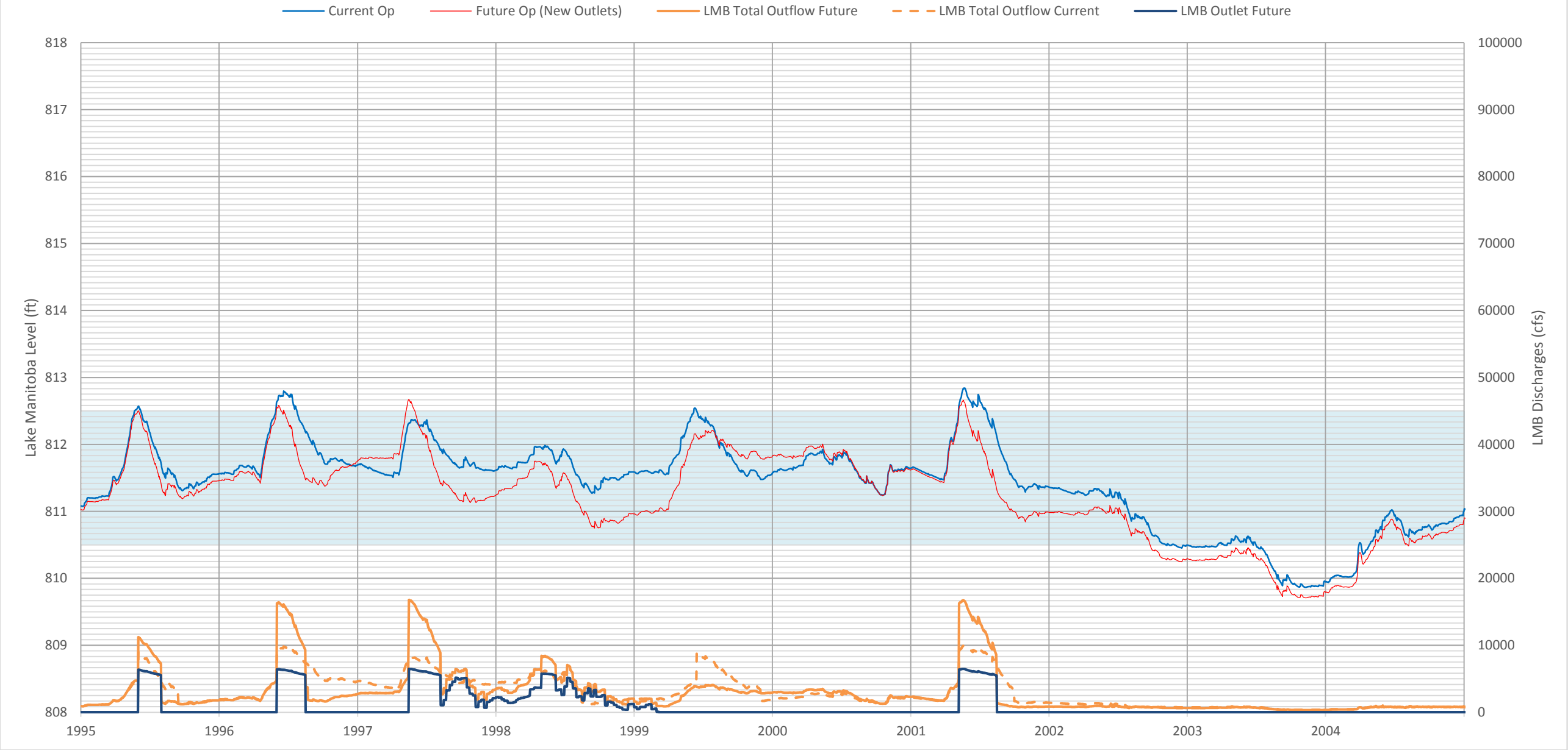
Lake Manitoba Water Level Simulations 1995 - 2004
