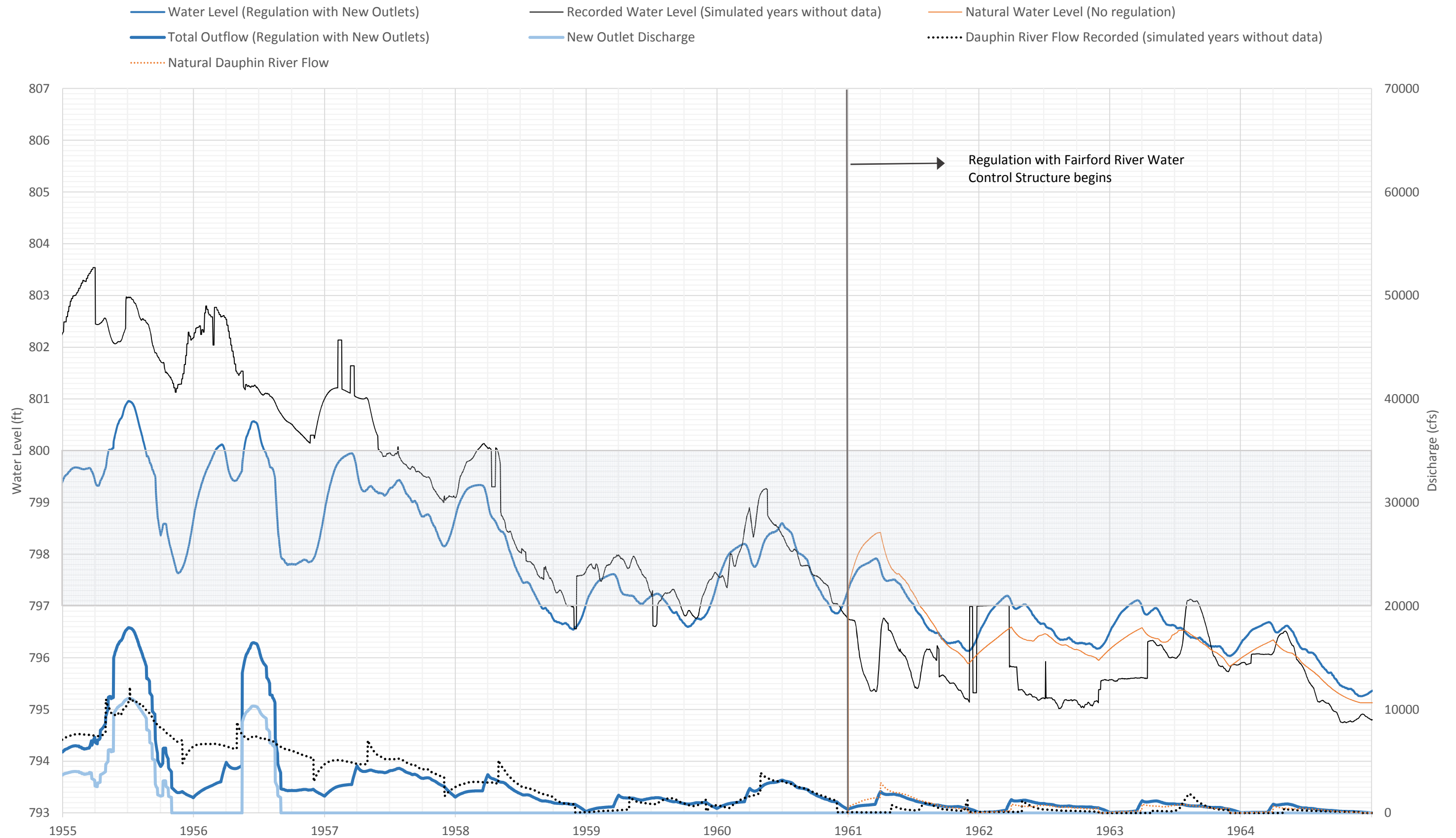
Lake St. Martin Water Levels and Outflows
