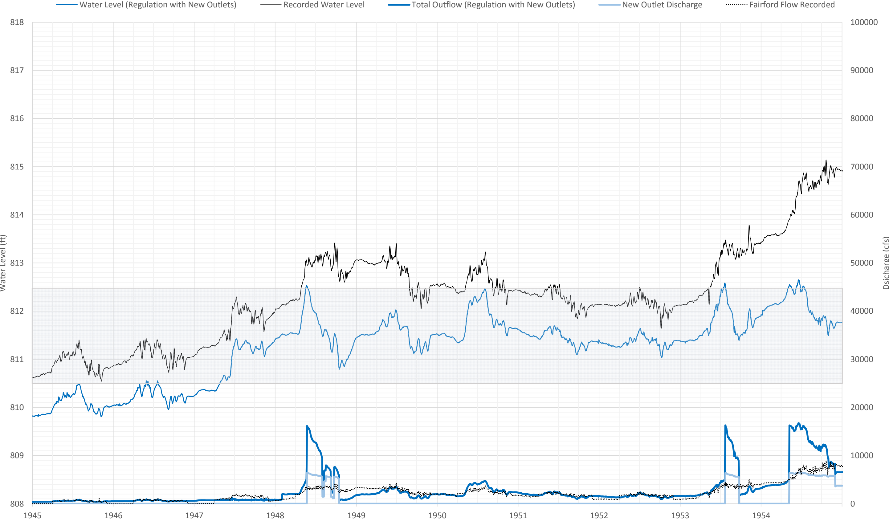
Lake Manitoba Water Levels and Outflows
