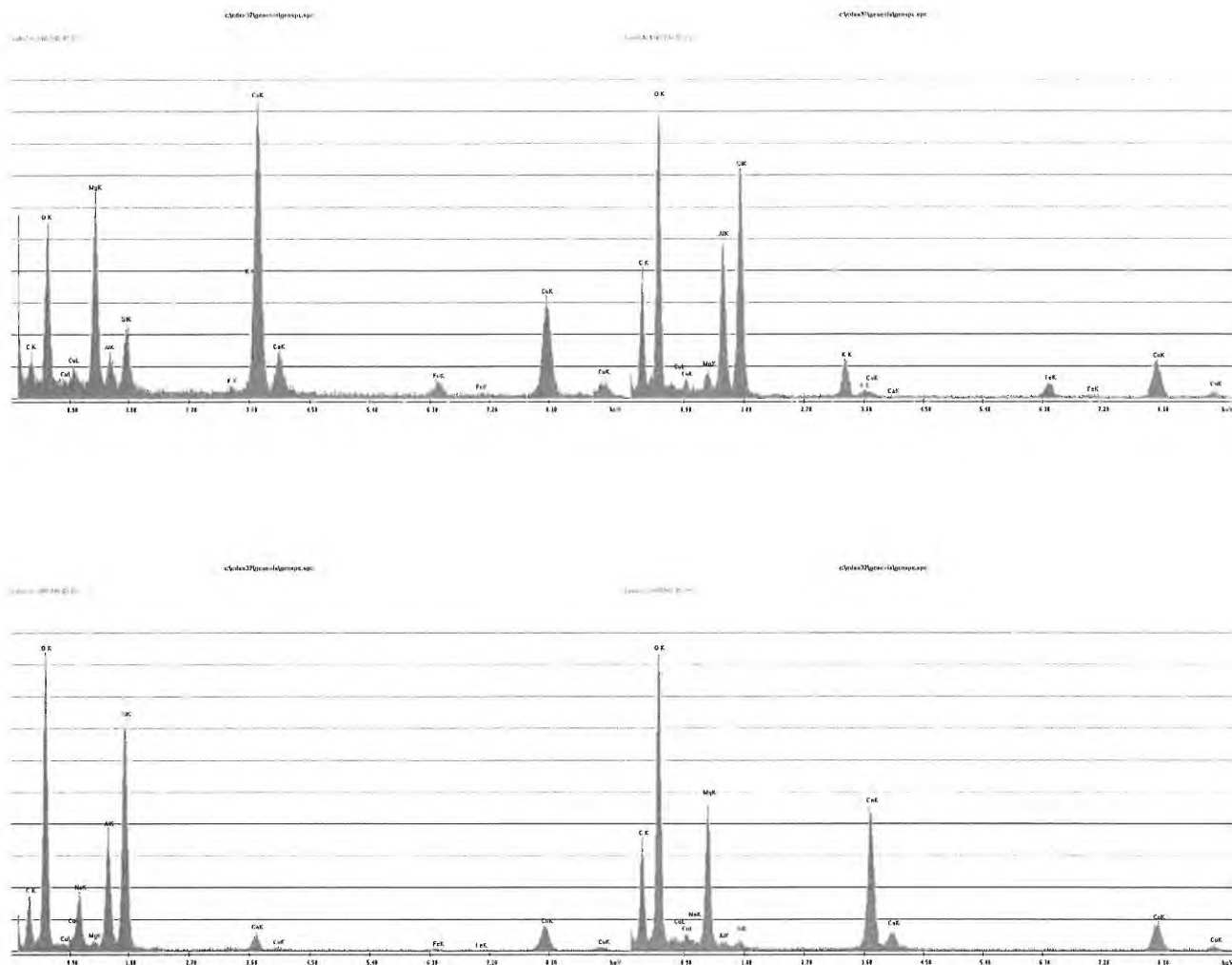
Representative EDXA Spectra
