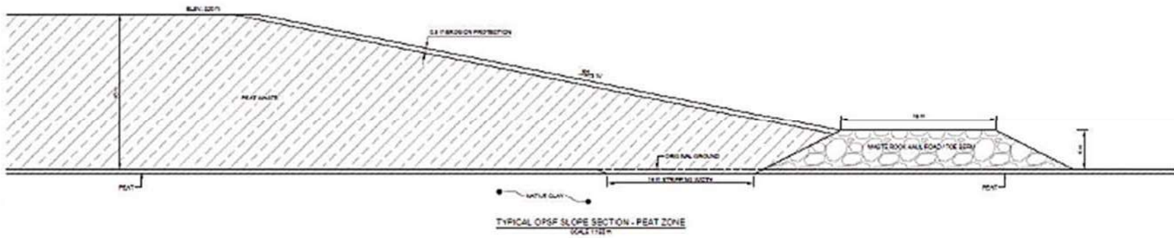
Figure 3 Cross-sections of the unconsolidated deposits and organic matter stockpile
