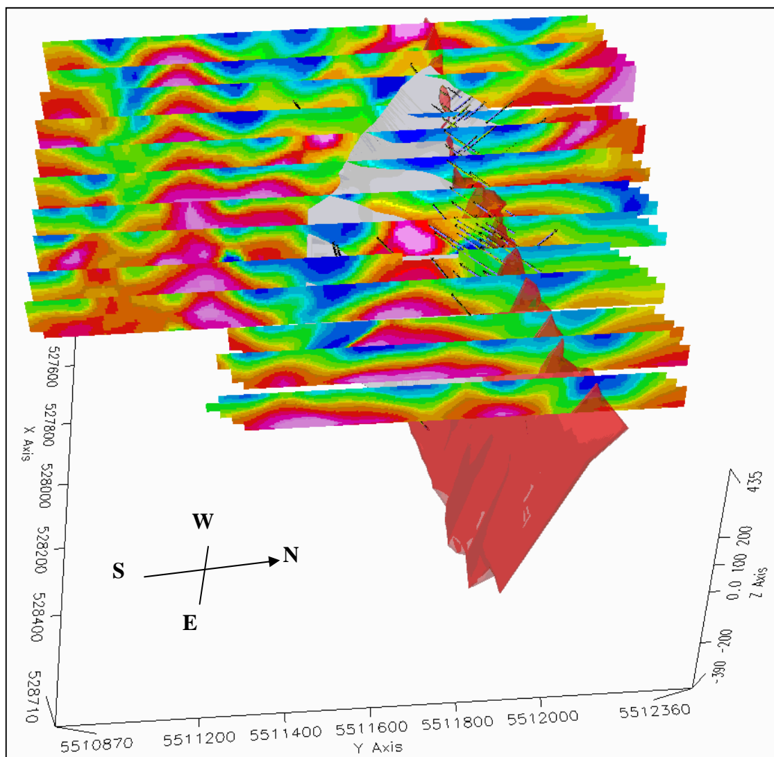
Figure 9-7. 3D view of Chargeability sections, fault (grey) possibly extends to west-northwest. Mineralized zone in red
