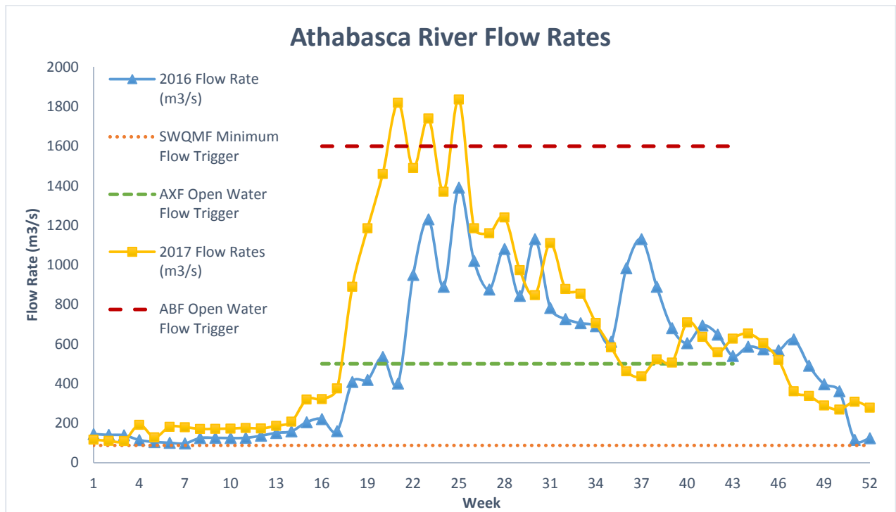
Figure 5-13: Weekly Athabasca River Flow Rates for 2016 and 2017 1
