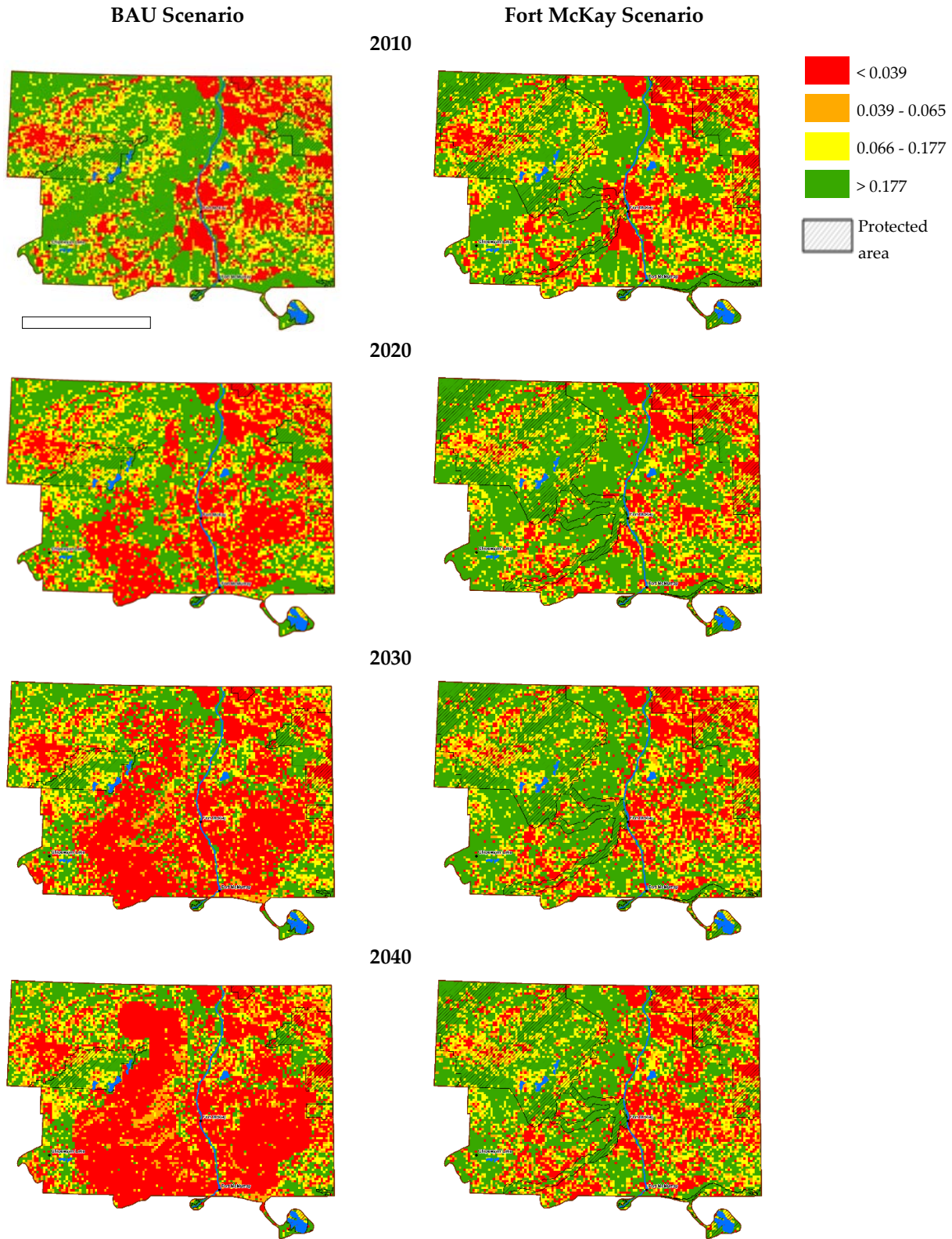
Figure 18: Projected future changes in fisher habitat suitability index values in the Business-as-Usual (BAU) and Fort McKay (FM) scenarios, years 2010-2040.
