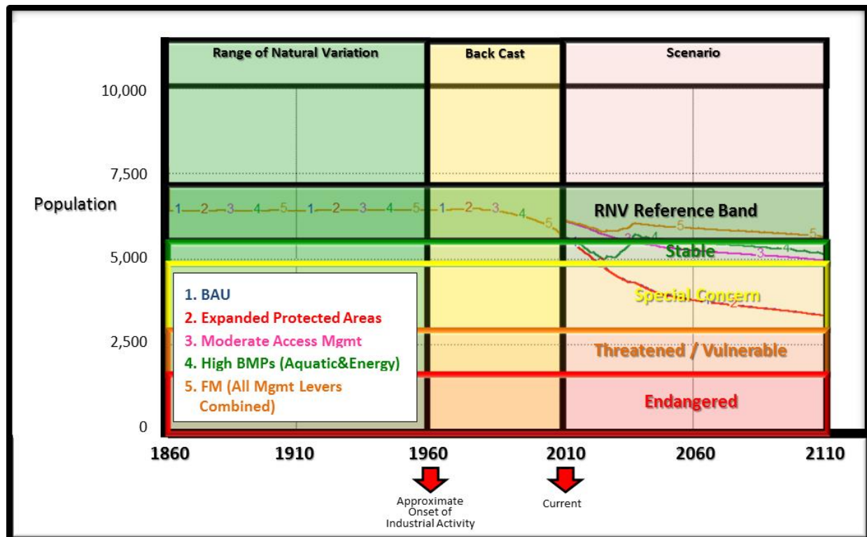
Figure 14: Patterns of moose HSI and population in the Business-as-Usual (BAU) and Fort McKay (FM) scenarios. The bottom graph shows risk bands.
