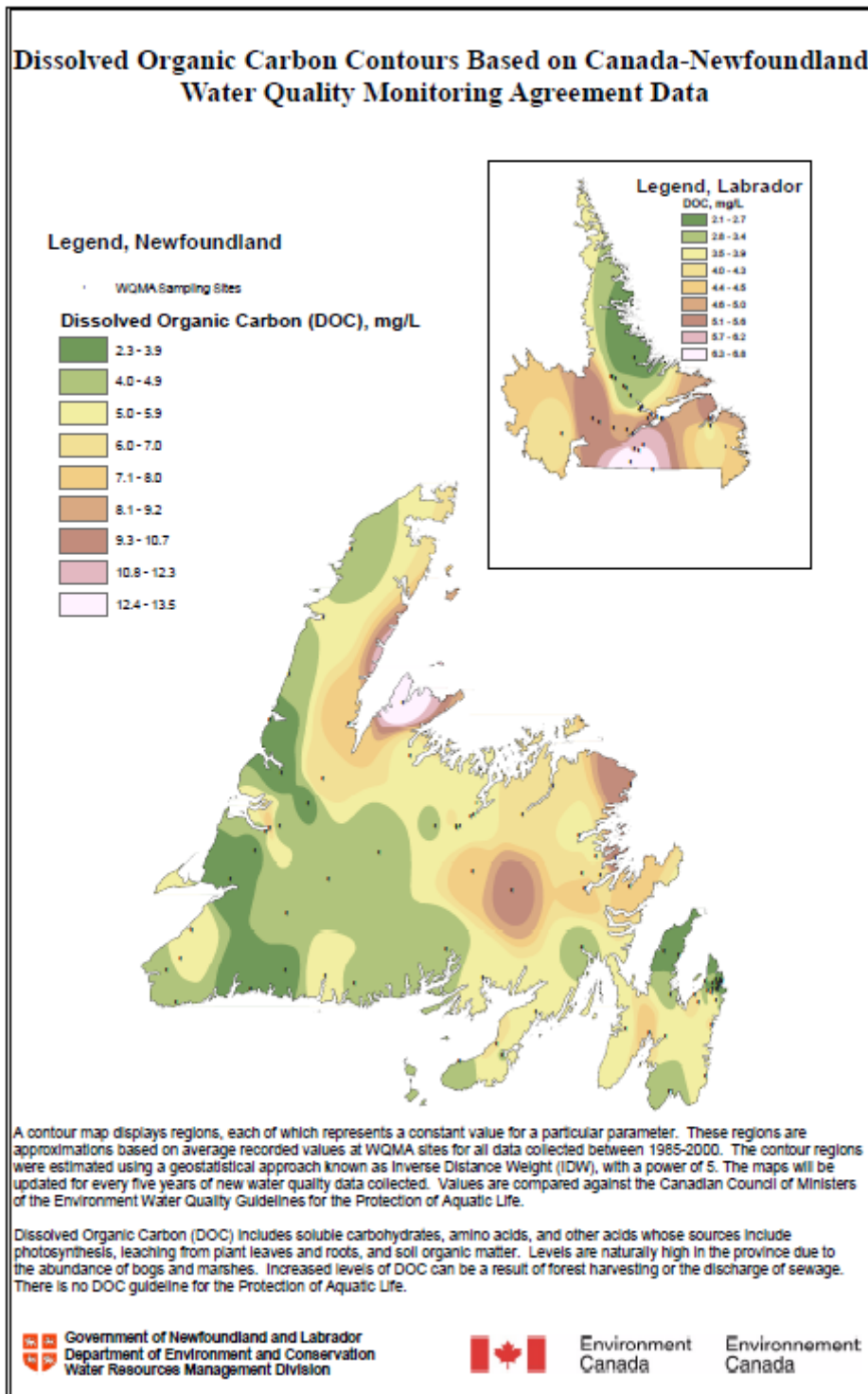
Figure 171.15 Dissolved Organic Carbon Contours Based on Canada-Newfoundland Water Quality Monitoring Agreement Data
