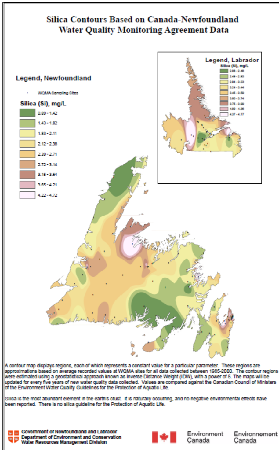
Figure 171.18 Silica Contours Based on Canada-Newfoundland Water Quality Monitoring Agreement Data
