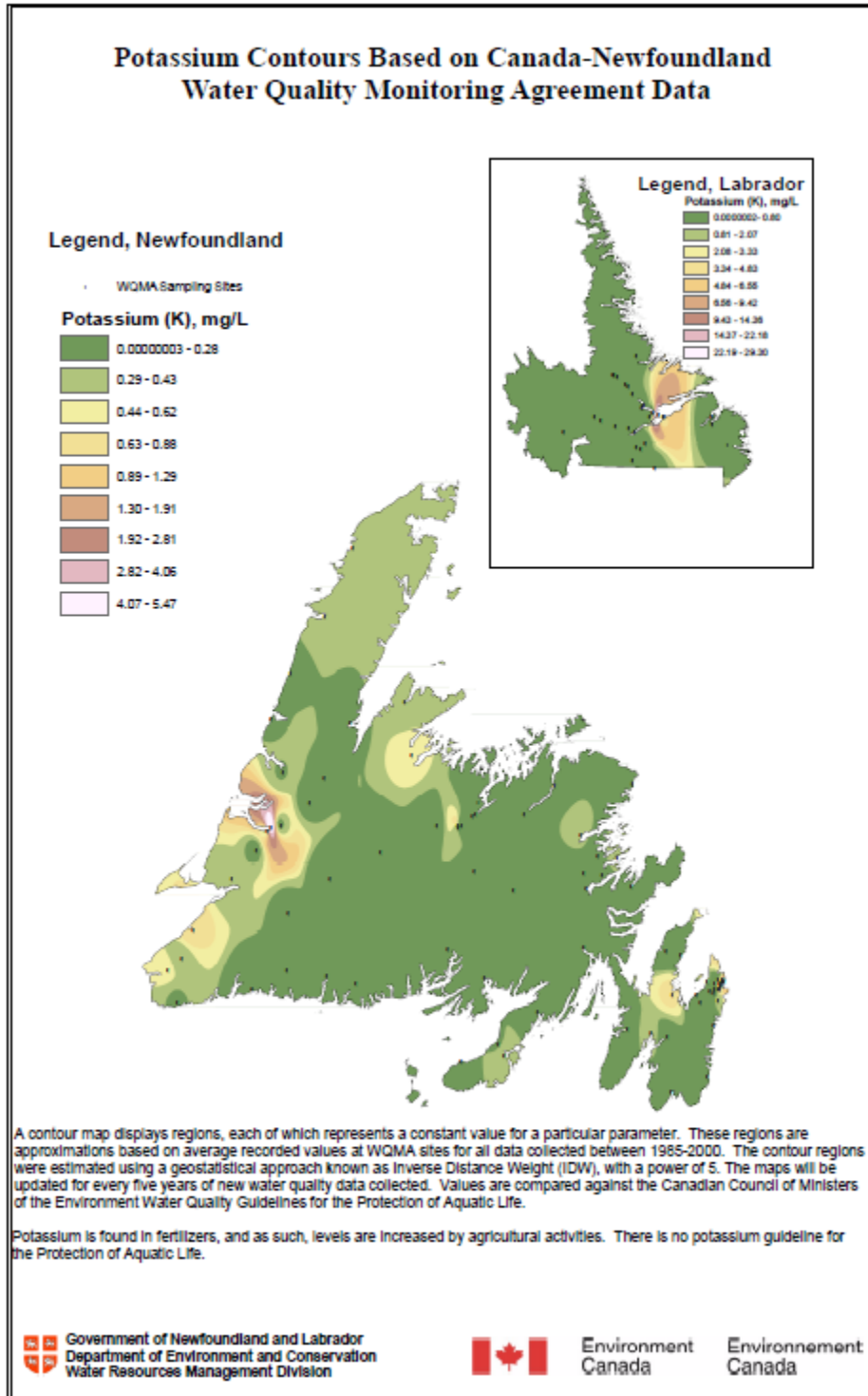
Figure 17I.12 Potassium Contours Based on Canada-Newfoundland Water Quality Monitoring Agreement Data
