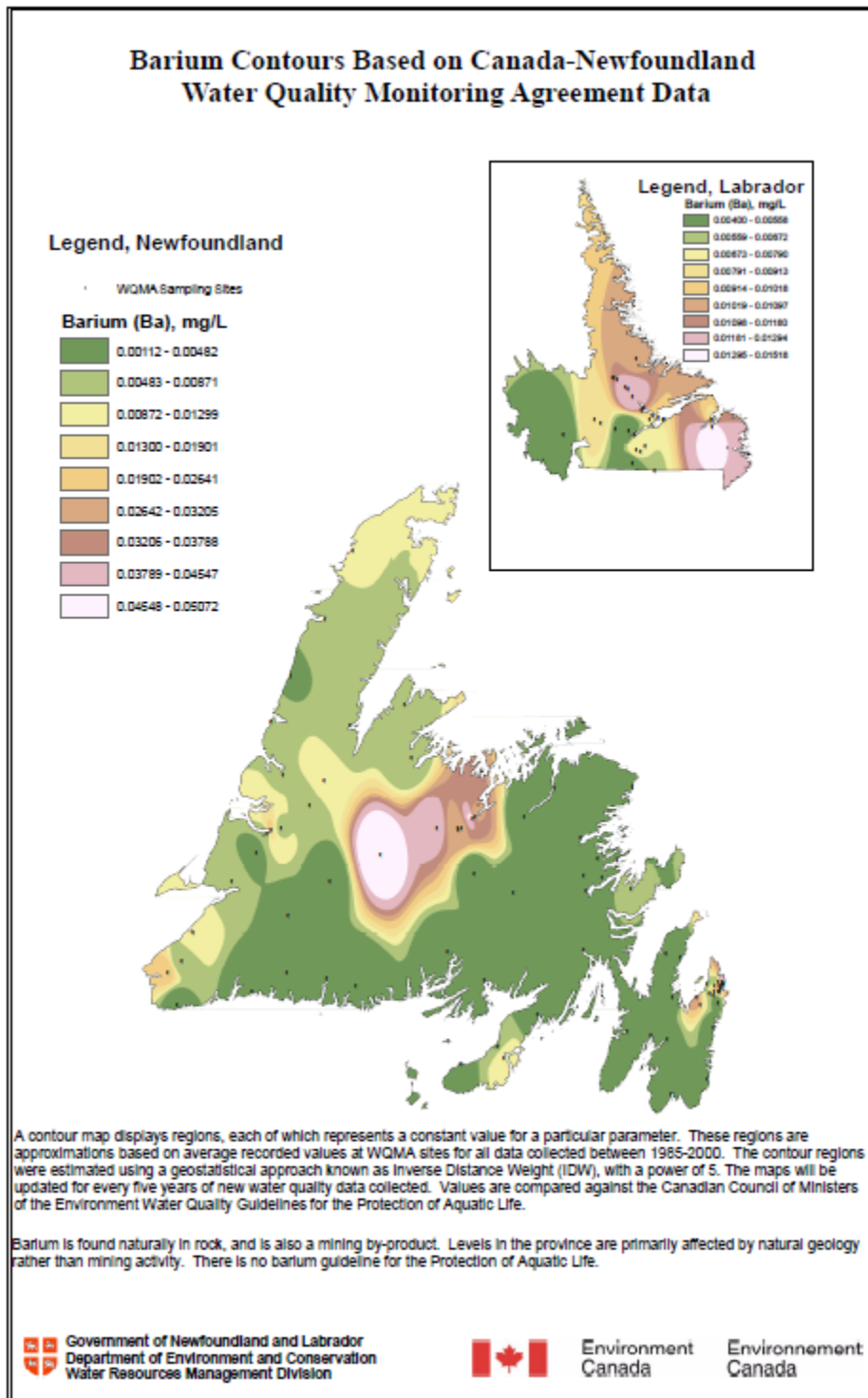
Figure 171.21 Barium Contours Based on Canada-Newfoundland Water Quality Monitoring Agreement Data
