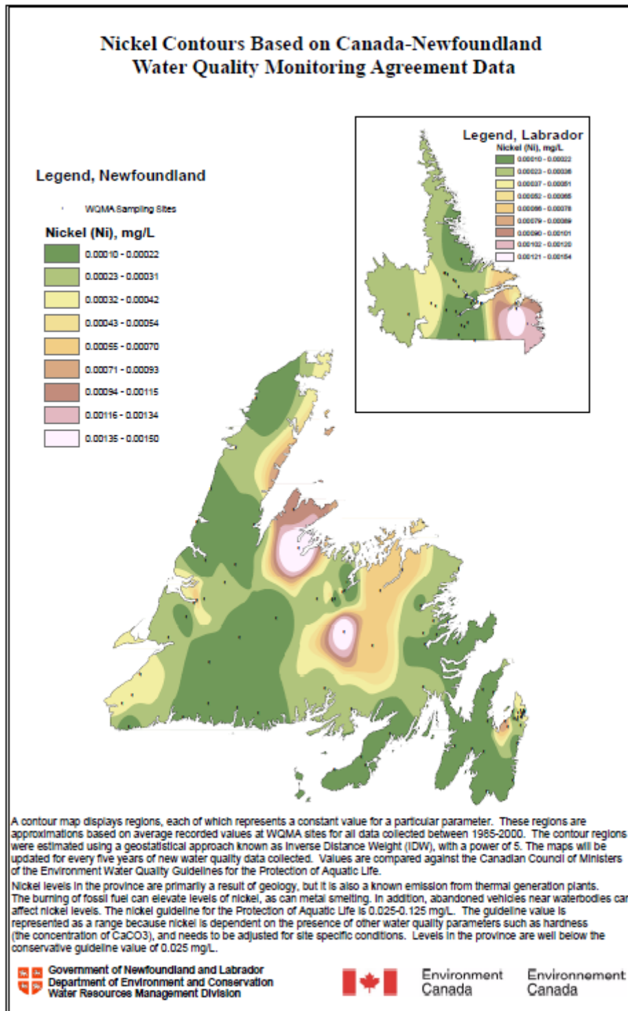
Figure 171.33 Nickel Contours Based on Canada-Newfoundland Water Quality Monitoring Agreement Data
