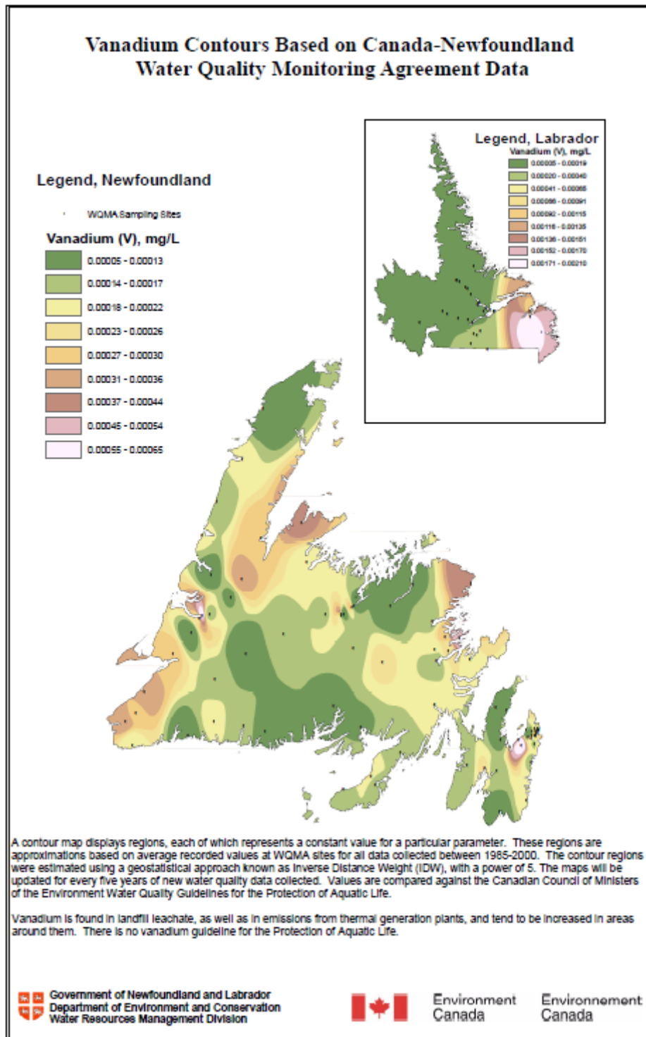
Figure 171.36 Vanadium Contours Based on Canada-Newfoundland Water Quality Monitoring Agreement Data
