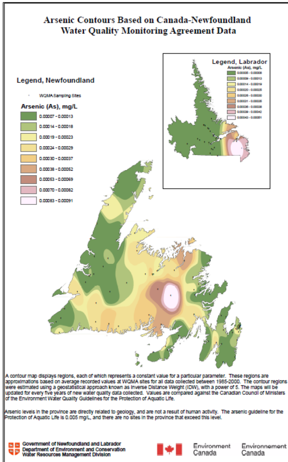
Figure 171.20 Arsenic Contours Based on Canada-Newfoundland Water Quality Monitoring Agreement Data
