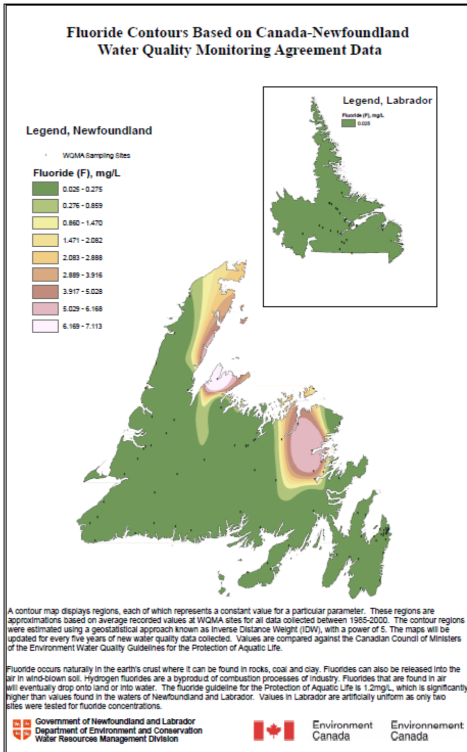
Figure 17I.10 Fluoride Contours Based on Canada-Newfoundland Water Quality Monitoring Agreement Data
