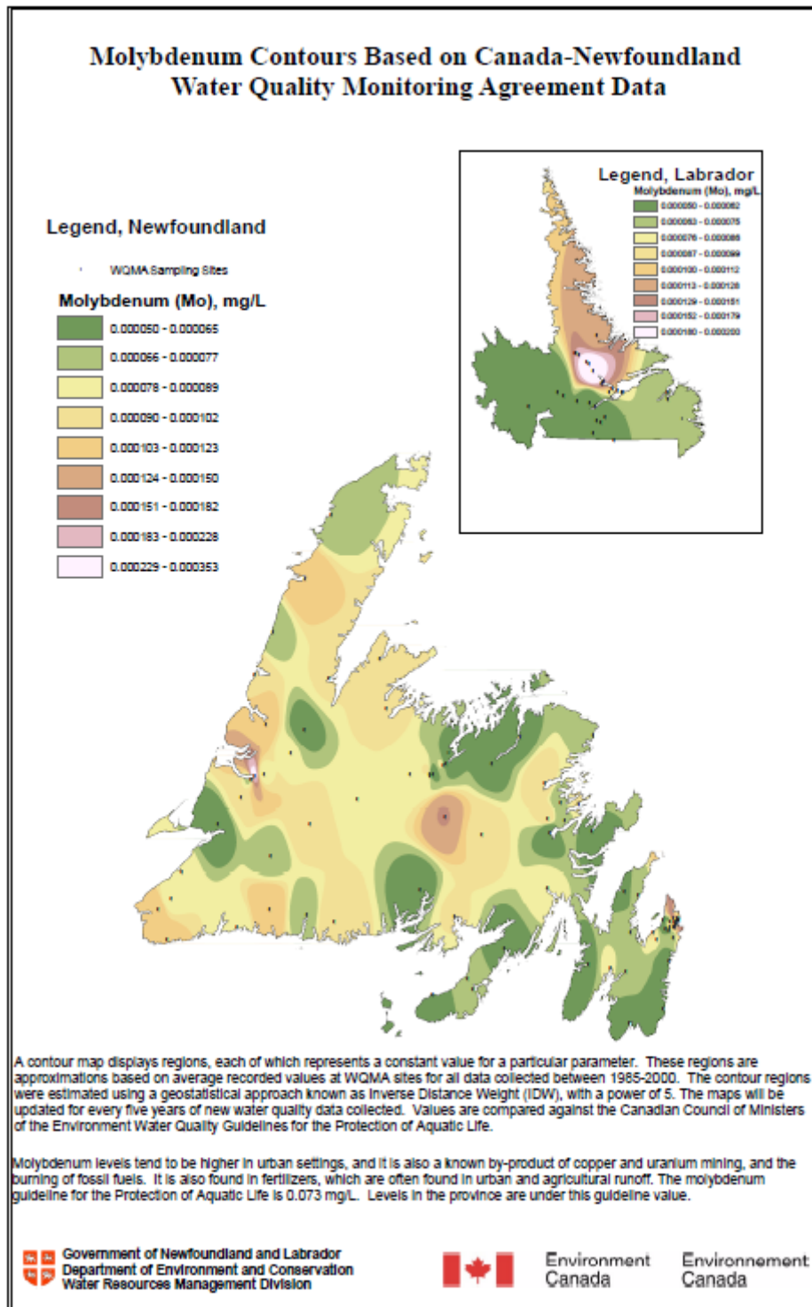
Figure 17I.32 Molybdenum Contours Based on Canada-Newfoundland Water Quality Monitoring Agreement Data
