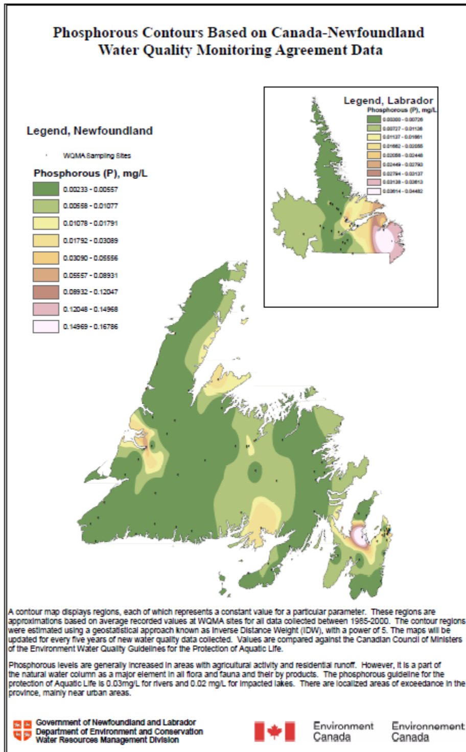
Figure 17I.17 Phosphorous Contours Based on Canada-Newfoundland Water Quality Monitoring Agreement Data
