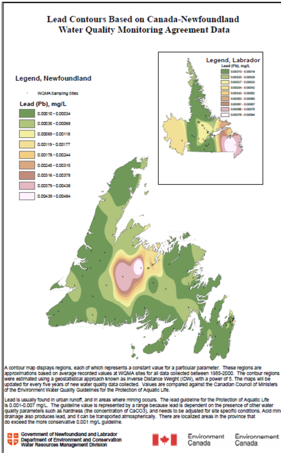
Figure 17I.28 Lead Contours Based on Canada-Newfoundland Water Quality Monitoring Agreement Data
