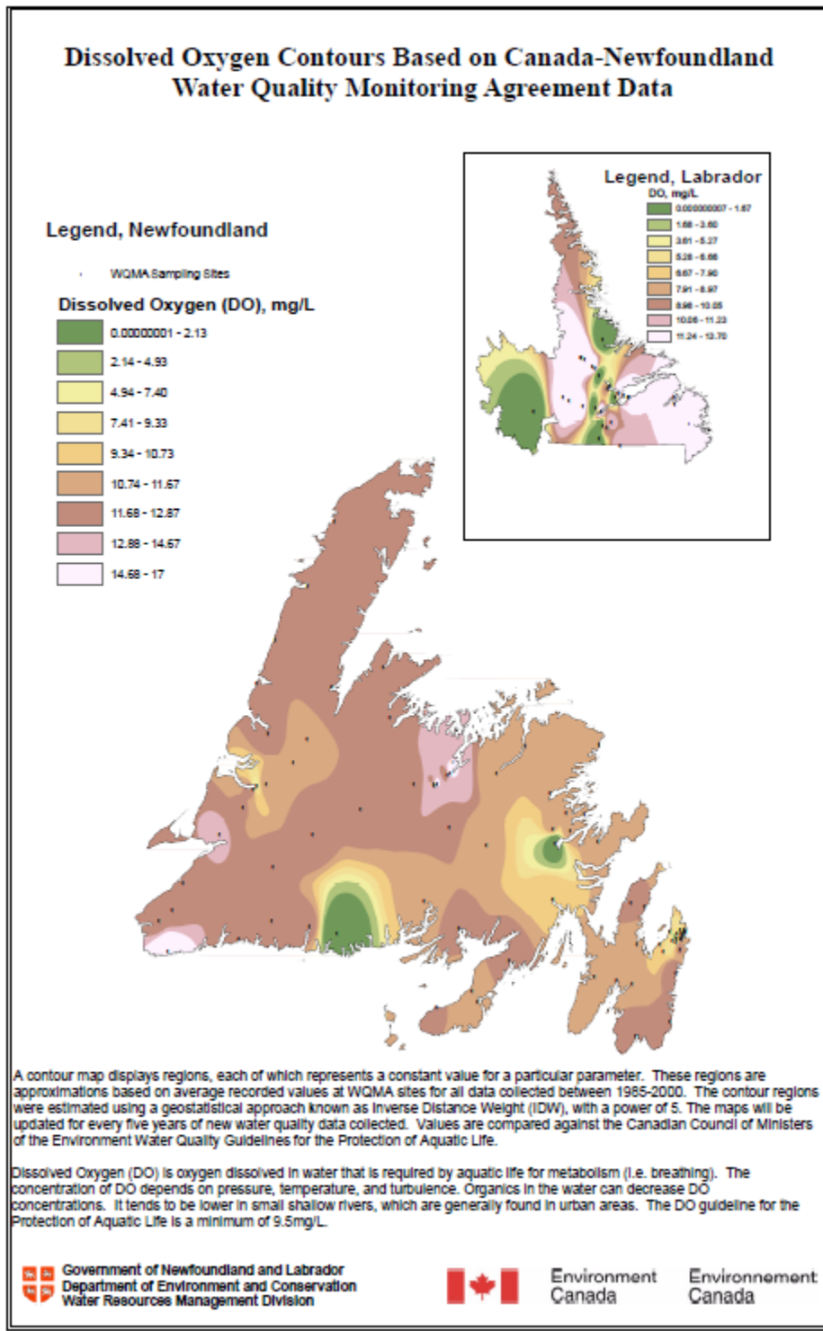
Figure 17I.4 Dissolved Oxygen Contours Based on Canada-Newfoundland Water Quality Monitoring Agreement Data
