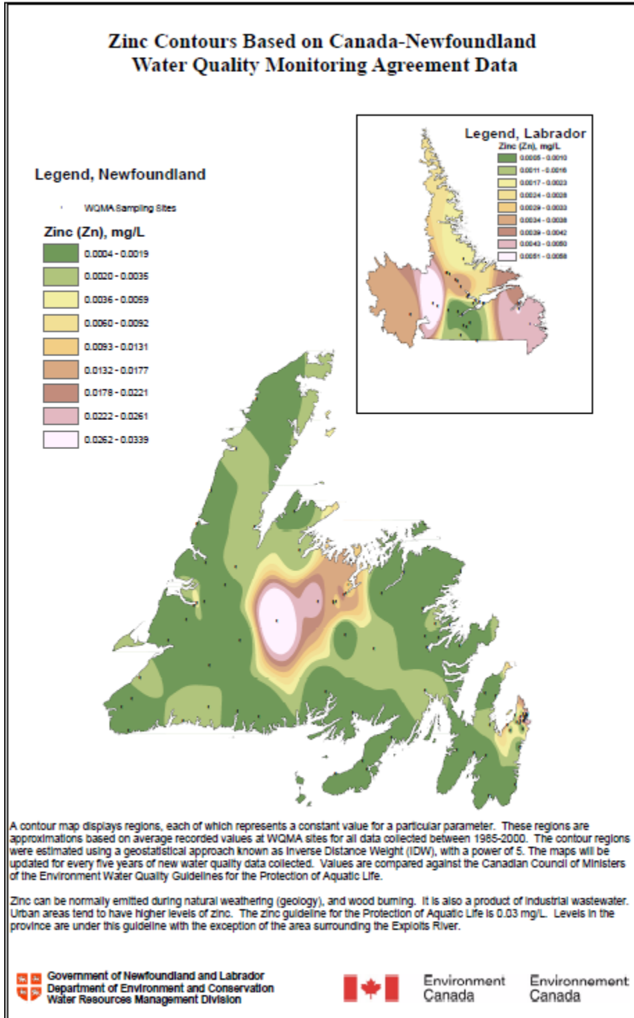
Figure 171.37 Zinc Contours Based on Canada-Newfoundland Water Quality Monitoring Agreement Data
