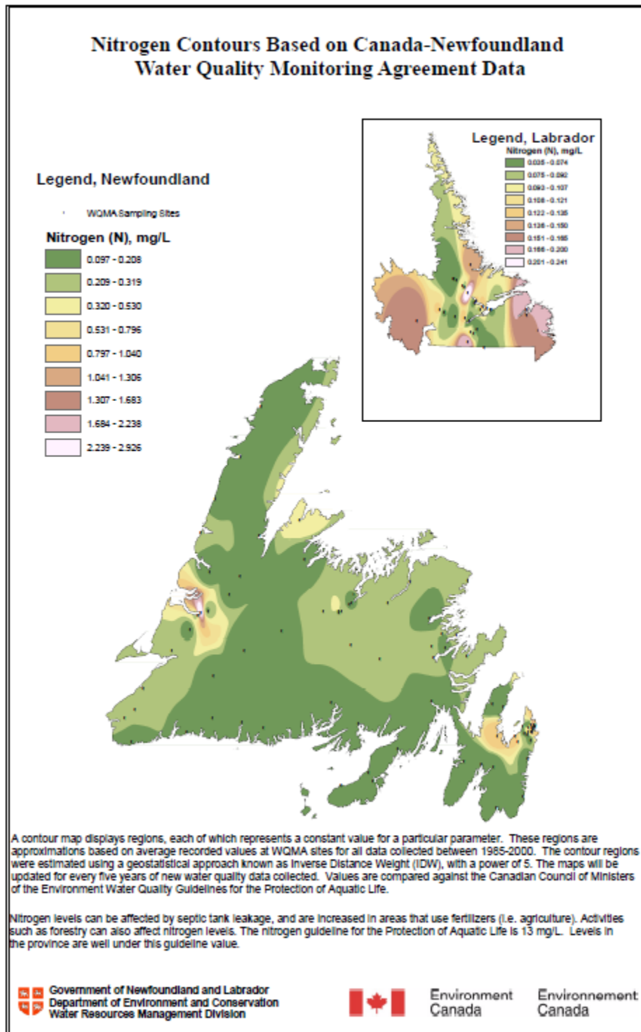
Figure 17I.16 Nitrogen Contours Based on Canada-Newfoundland Water Quality Monitoring Agreement Data
