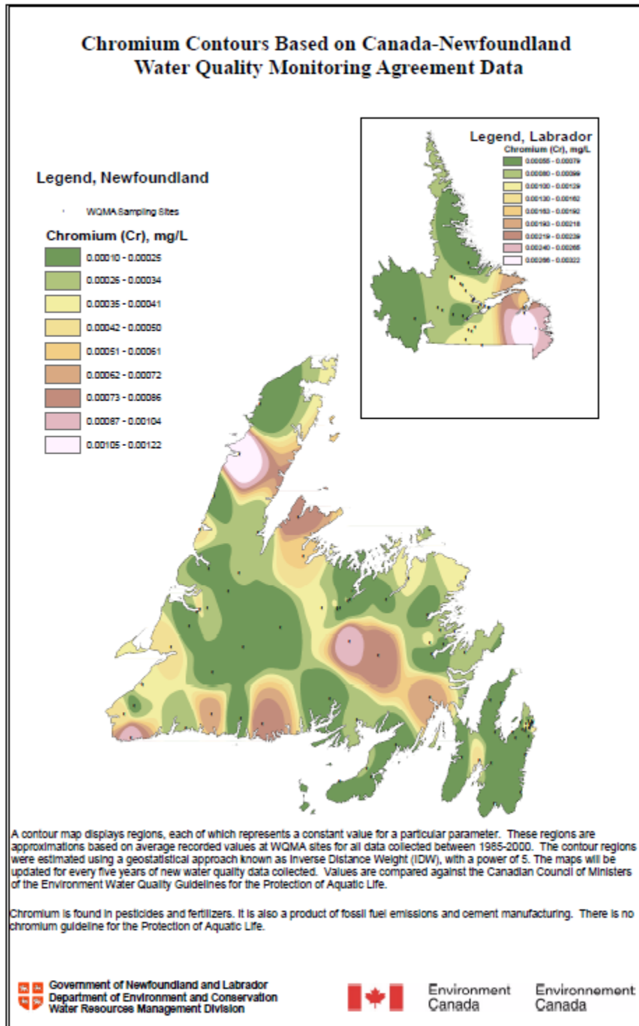
Figure 17I.25 Chromium Contours Based on Canada-Newfoundland Water Quality Monitoring Agreement Data
