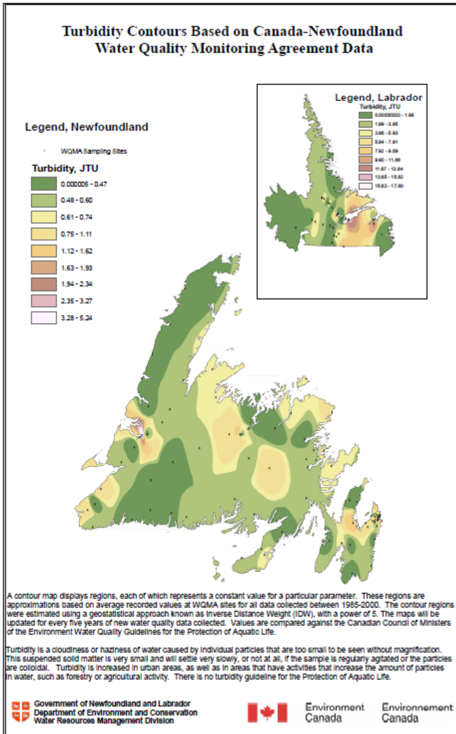
Figure 171.6 Turbidity Contours Based on Canada-Newfoundland Water Quality Monitoring Agreement Data
