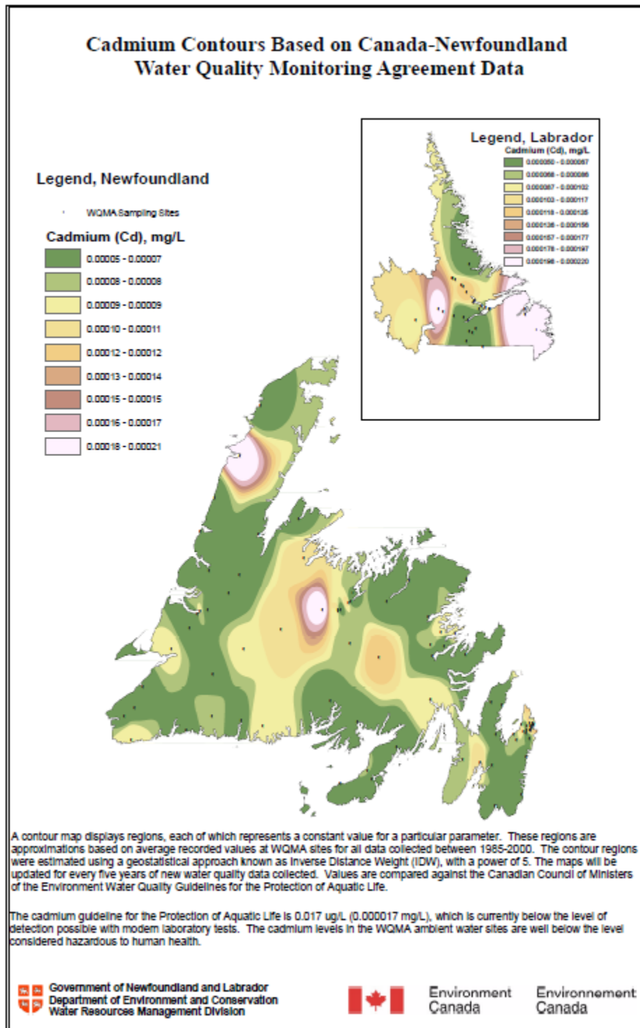
Figure 171.23 Cadmium Contours Based on Canada-Newfoundland Water Quality Monitoring Agreement Data
