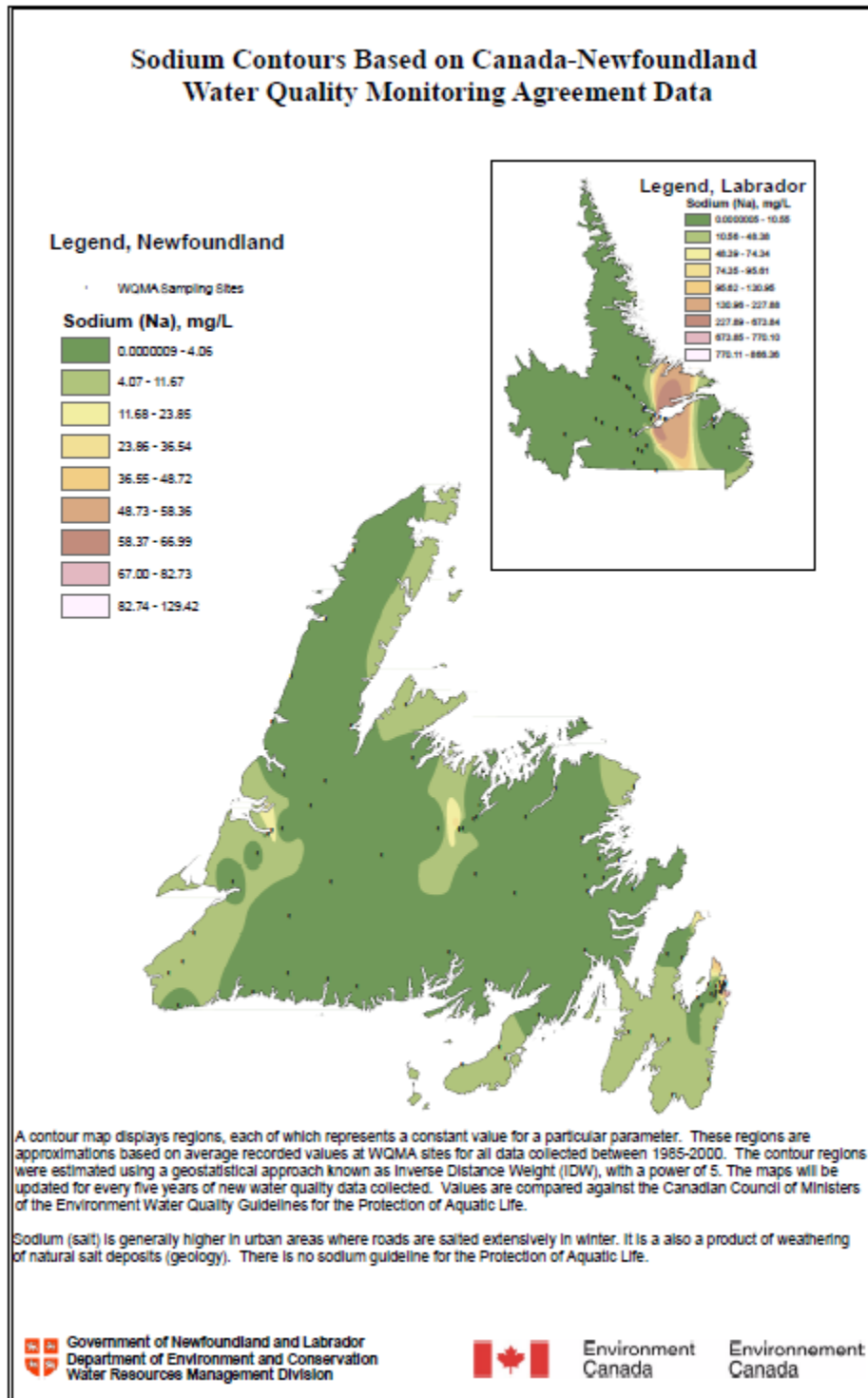
Figure 171.13 Sodium Contours Based on Canada-Newfoundland Water Quality Monitoring Agreement Data
