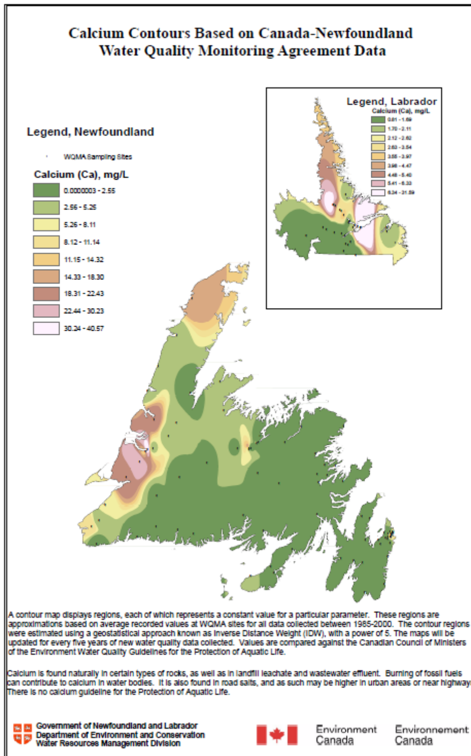
Figure 171.8 Calcium Contours Based on Canada-Newfoundland Water Quality Monitoring Agreement Data
