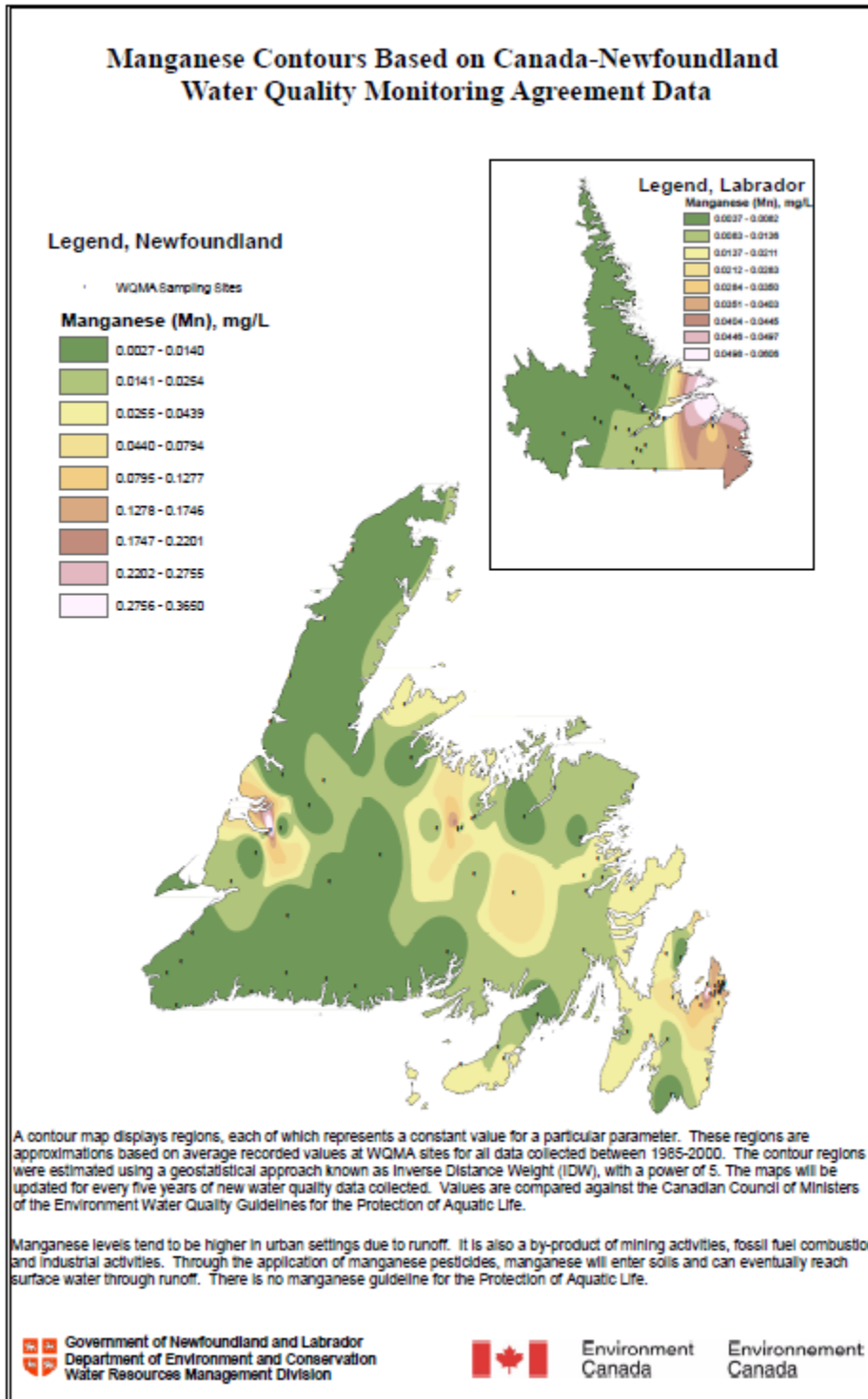
Figure 17I.30 Manganese Contours Based on Canada-Newfoundland Water Quality Monitoring Agreement Data
