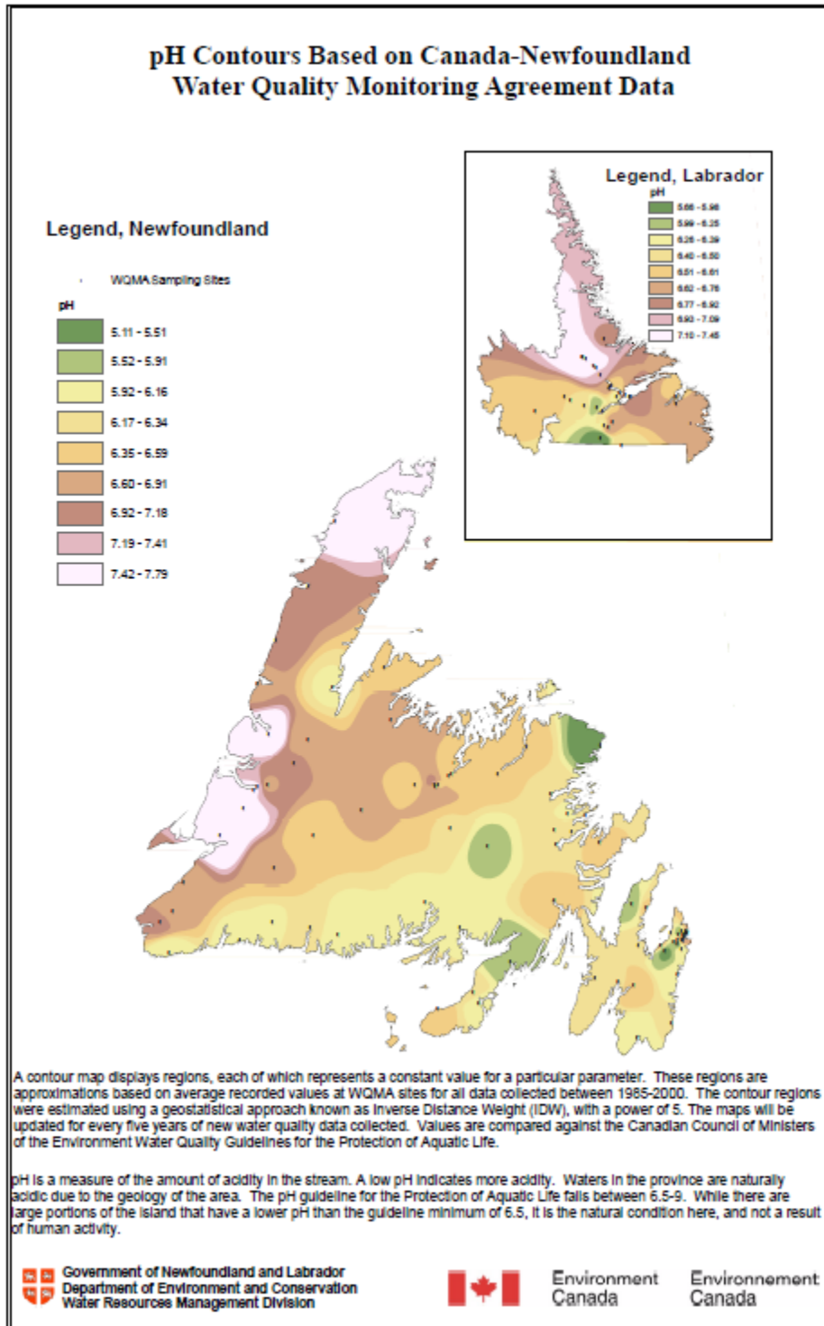
Figure 171.5 pH Contours Based on Canada-Newfoundland Water Quality Monitoring Agreement Data
