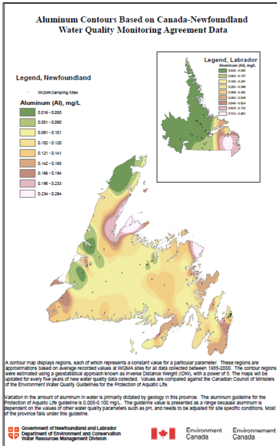
Figure 17I.19 Aluminum Contours Based on Canada-Newfoundland Water Quality Monitoring Agreement Data
