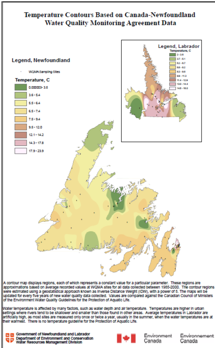
Figure 171.7 Temperature Contours Based on Canada-Newfoundland Water Quality Monitoring Agreement Data
