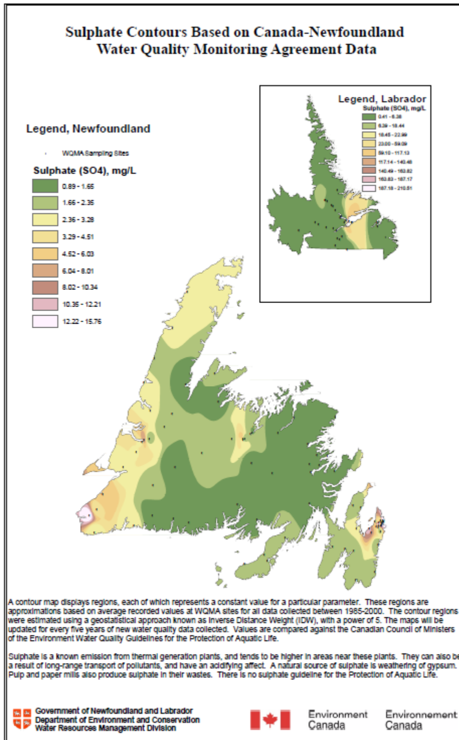
Figure 17I.14 Sulphate Contours Based on Canada-Newfoundland Water Quality Monitoring Agreement Data
