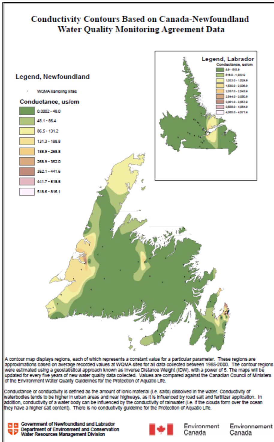
Figure 171.3 Conductivity Contours Based on Canada-Newfoundland Water Quality Monitoring Agreement Data
