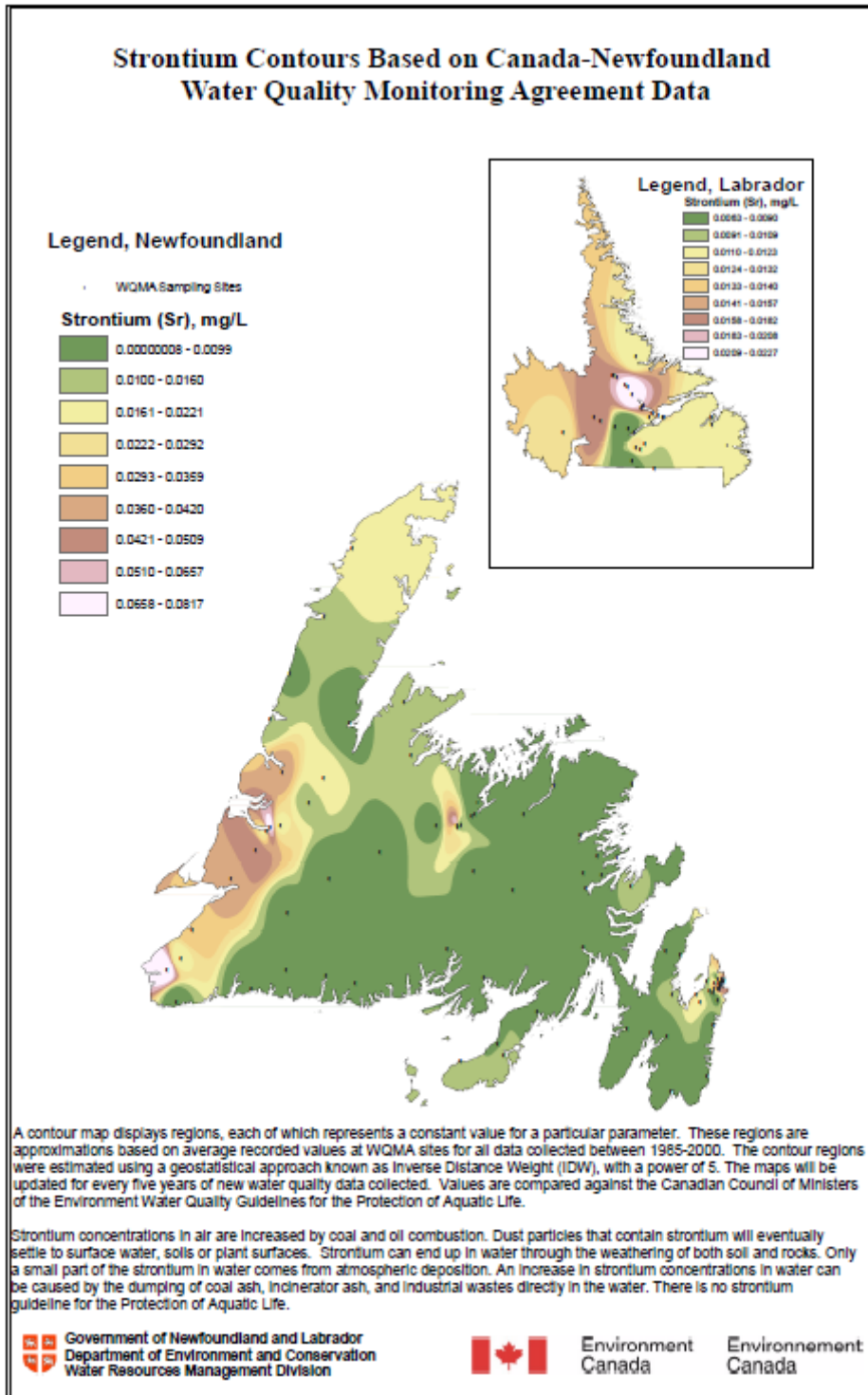
Figure 171.35 Strontium Contours Based on Canada-Newfoundland Water Quality Monitoring Agreement Data
