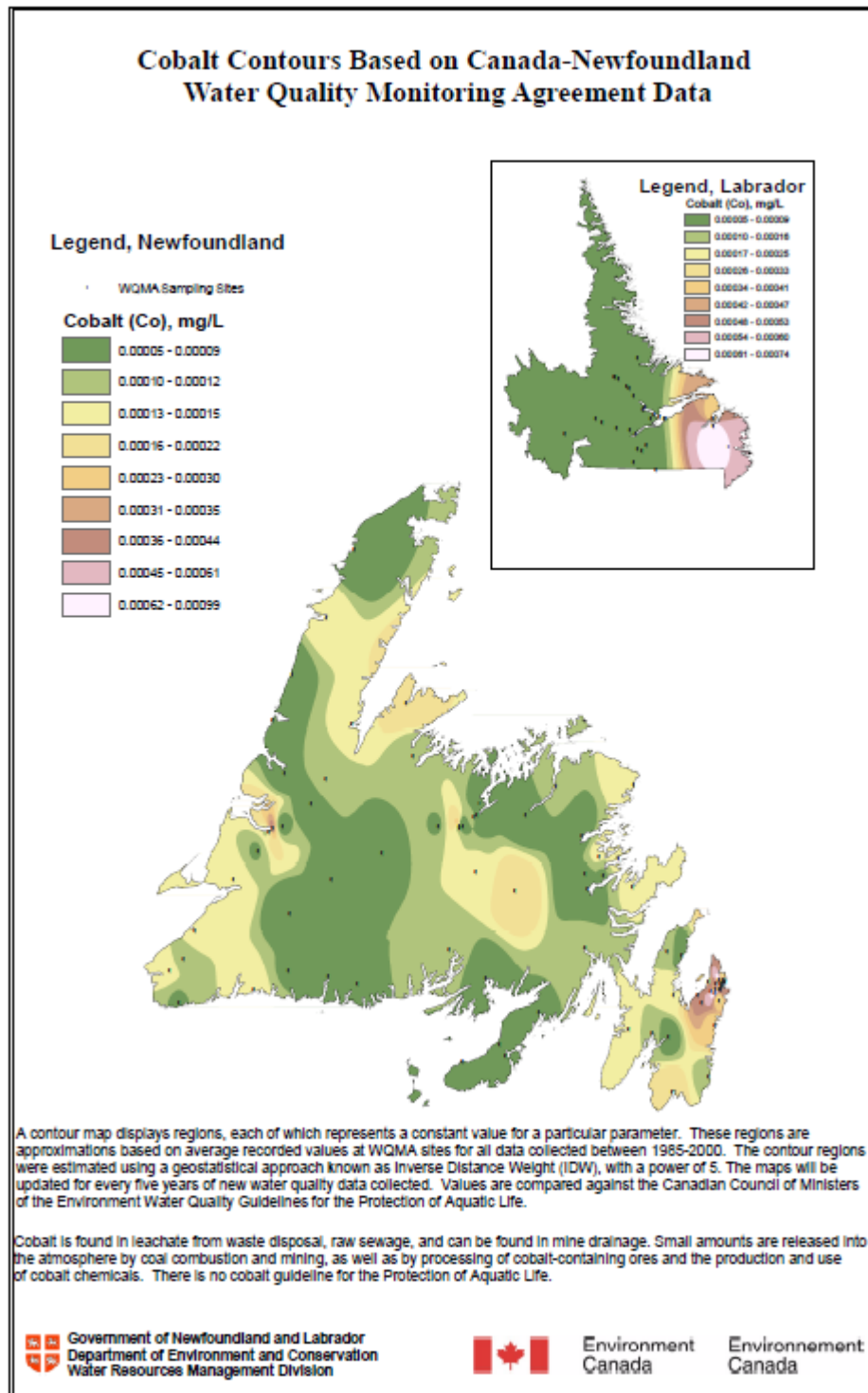
Figure 17I.24 Cobalt Contours Based on Canada-Newfoundland Water Quality Monitoring Agreement Data
