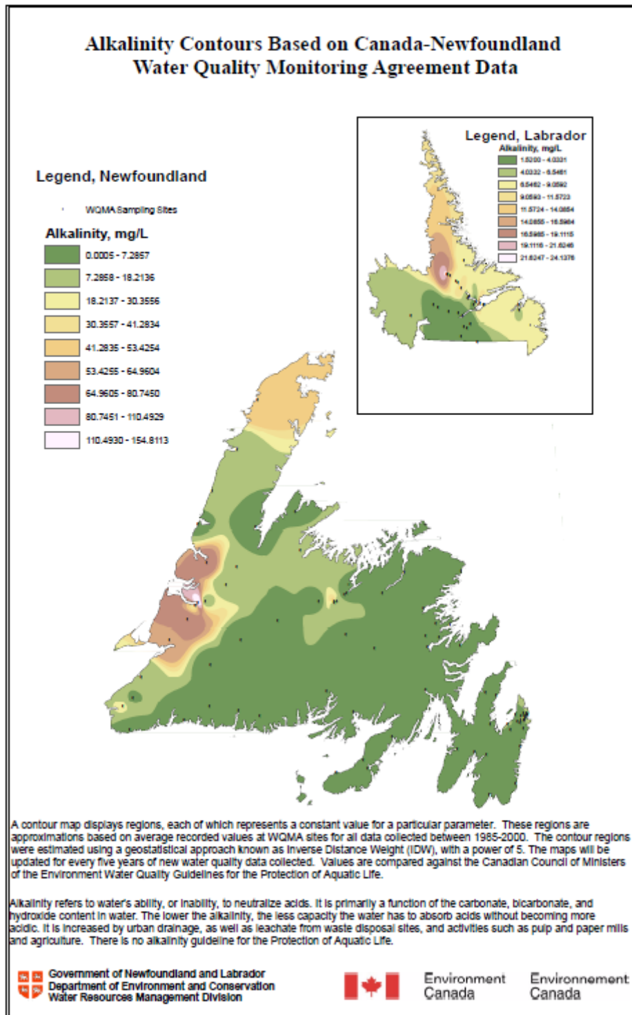
Figure 171.1 Alkalinity Contours Based on Canada-Newfoundland Water Quality Monitoring Agreement Data
