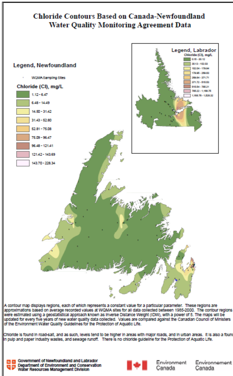
Figure 171.9 Chloride Contours Based on Canada-Newfoundland Water Quality Monitoring Agreement Data
