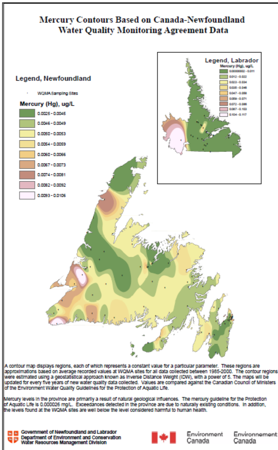
Figure 17I.31 Mercury Contours Based on Canada-Newfoundland Water Quality Monitoring Agreement Data
