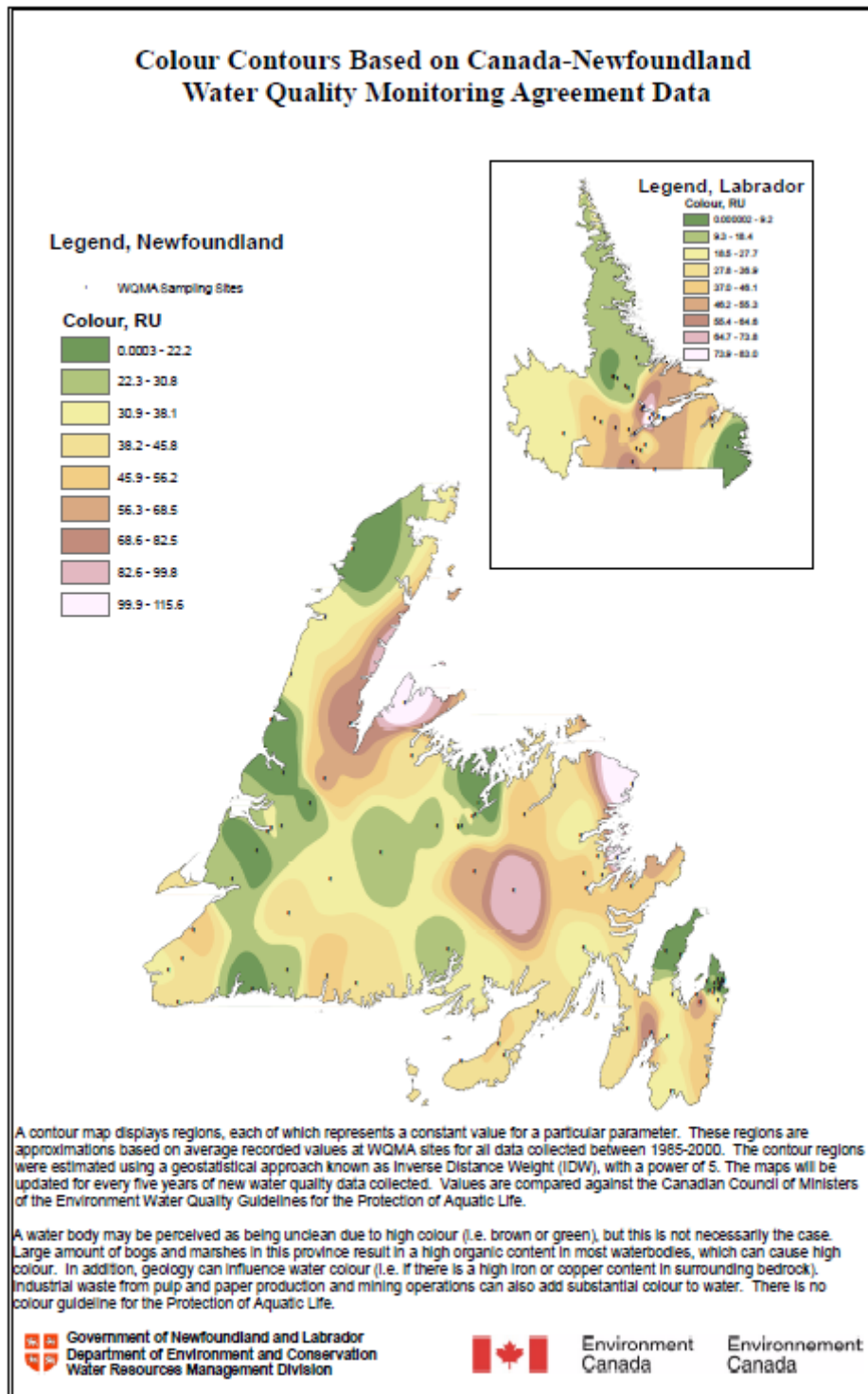
Figure 17I.2 Colour Contours Based on Canada-Newfoundland Water Quality Monitoring Agreement Data
