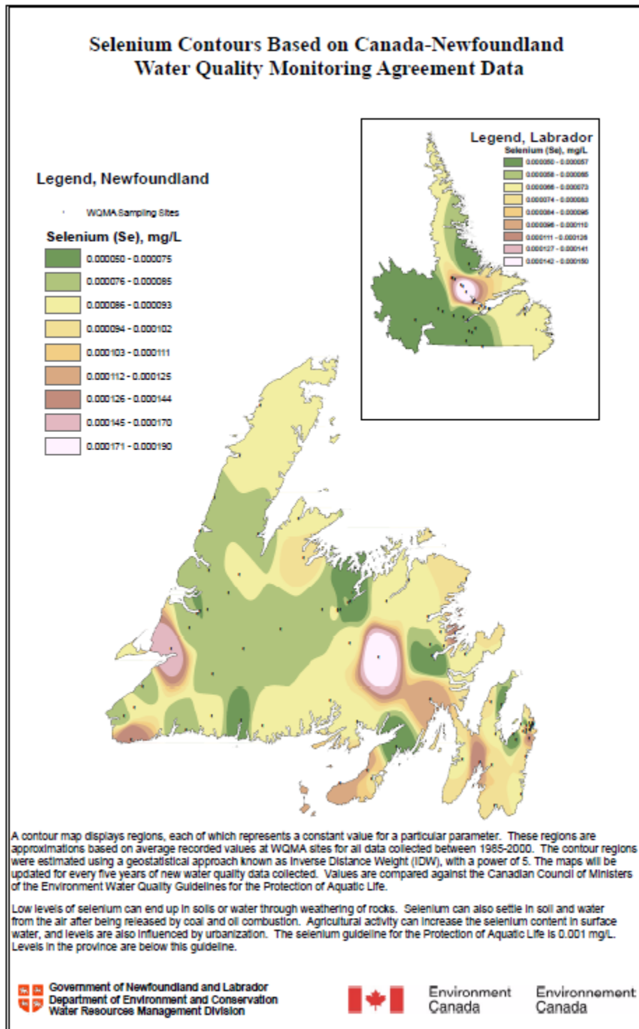
Figure 171.34 Selenium Contours Based on Canada-Newfoundland Water Quality Monitoring Agreement Data
