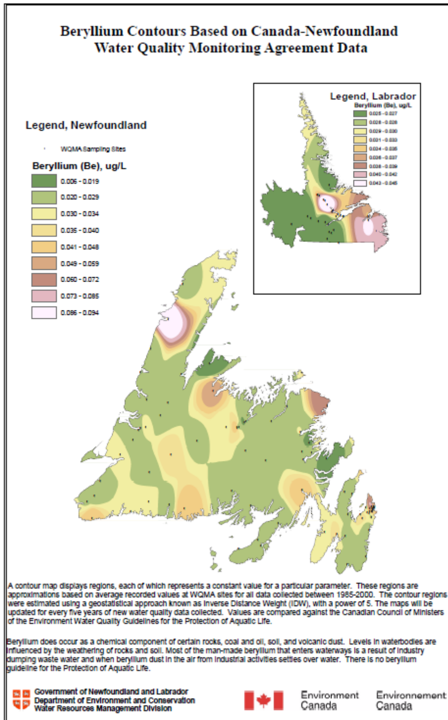
Figure 17I.22 Beryllium Contours Based on Canada-Newfoundland Water Quality Monitoring Agreement Data
