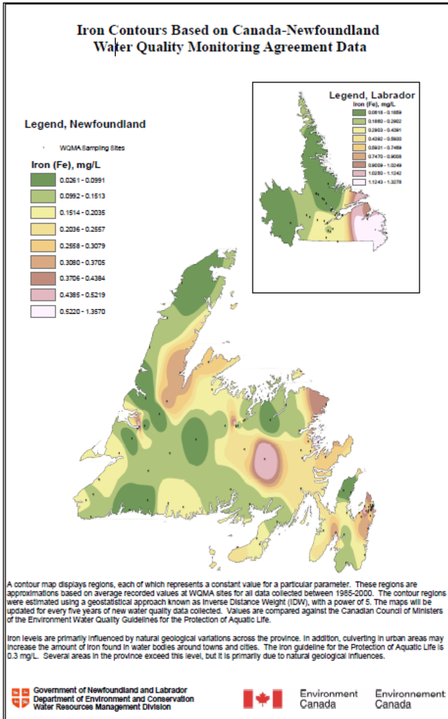
Figure 171.27 Iron Contours Based on Canada-Newfoundland Water Quality Monitoring Agreement Data
