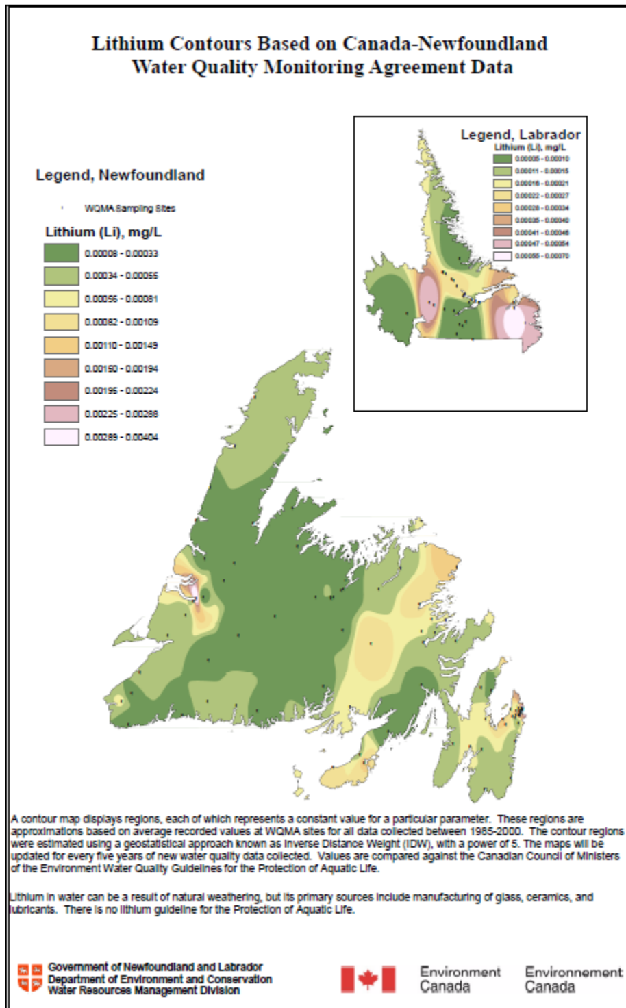
Figure 17I.29 Lithium Contours Based on Canada-Newfoundland Water Quality Monitoring Agreement Data
