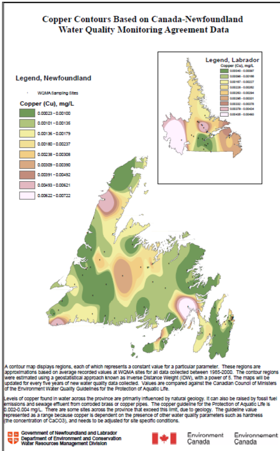
Figure 17I.26 Copper Contours Based on Canada-Newfoundland Water Quality Monitoring Agreement Data
