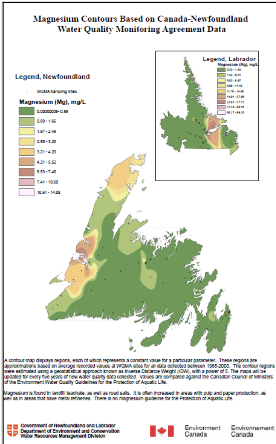
Figure 17I.11 Magnesium Contours Based on Canada-Newfoundland Water Quality Monitoring Agreement Data
